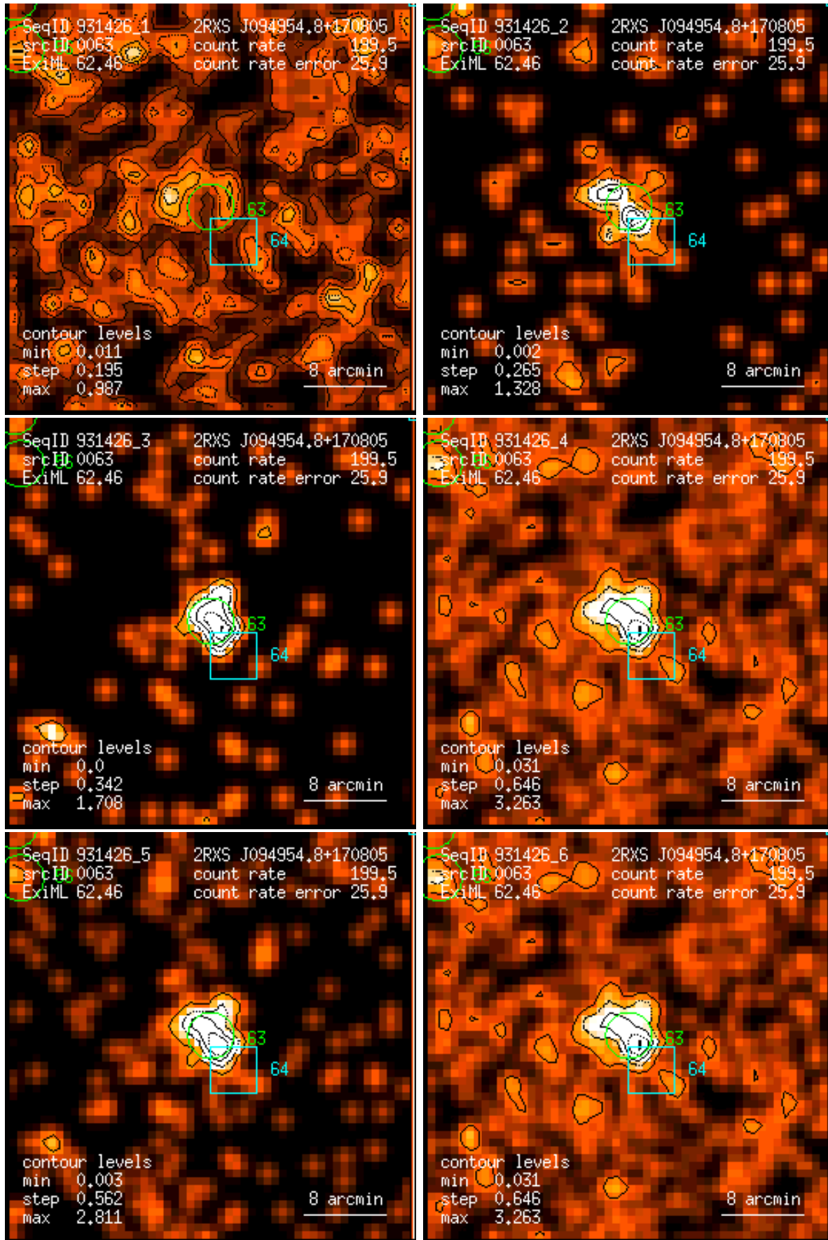
Figure 63: RASS 931426: detection 0063: band rate images, Gaussian filter: (1) PSPC channels 11 – 41, (2) 52 – 90, (3) 91 – 201, (4) 11 – 235, (5) 52 – 201, (6) 11 – 201. Broad band rates in counts/ks. Band rate contour levels in counts/ks/arcmin 2 .
