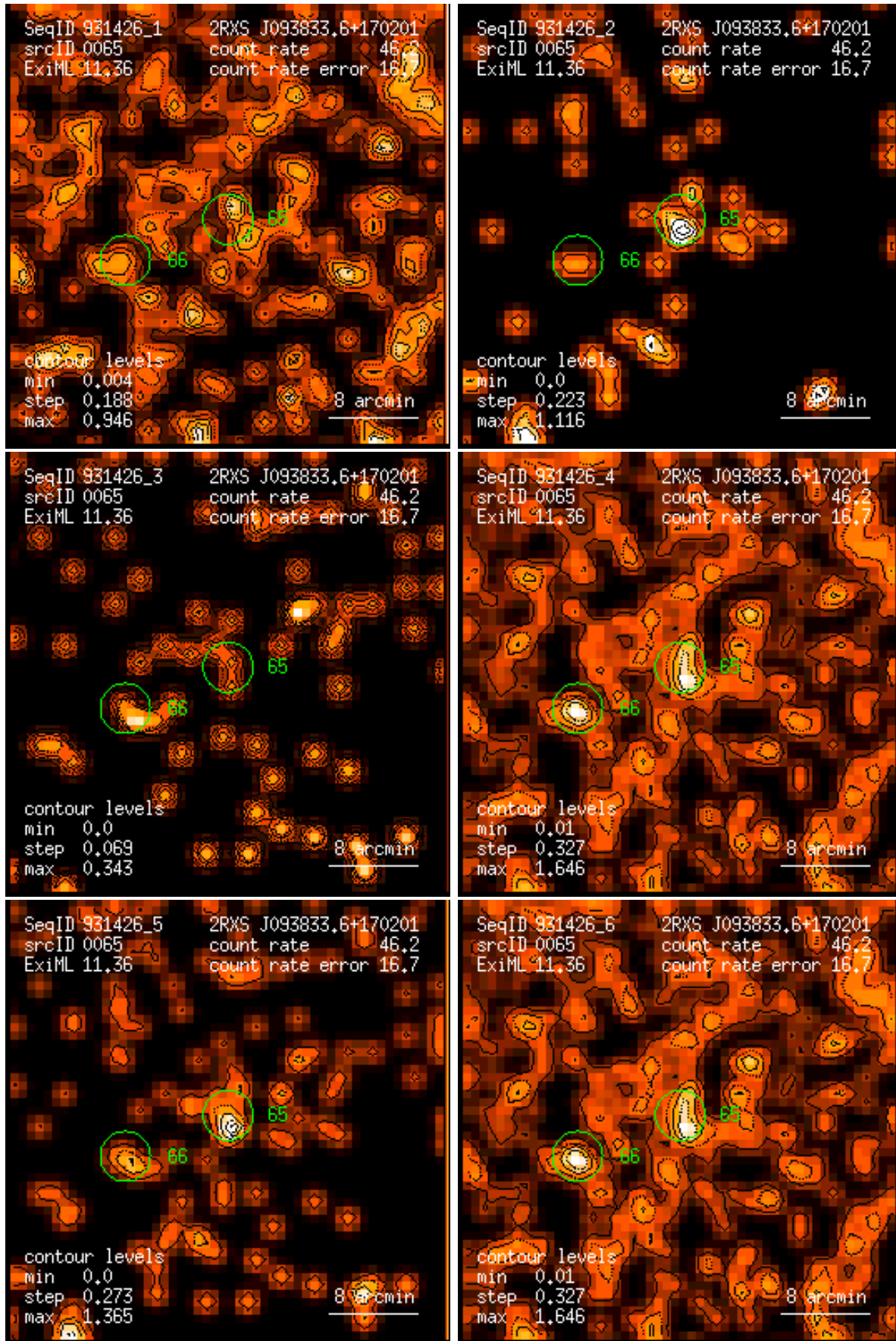
Figure 65: RASS 931426: detection 0065: band rate images, Gaussian filter: (1) PSPC channels 11 – 41, (2) 52 – 90, (3) 91 – 201, (4) 11 – 235, (5) 52 – 201, (6) 11 – 201. Broad band rates in counts/ks. Band rate contour levels in counts/ks/arcmin 2 .
