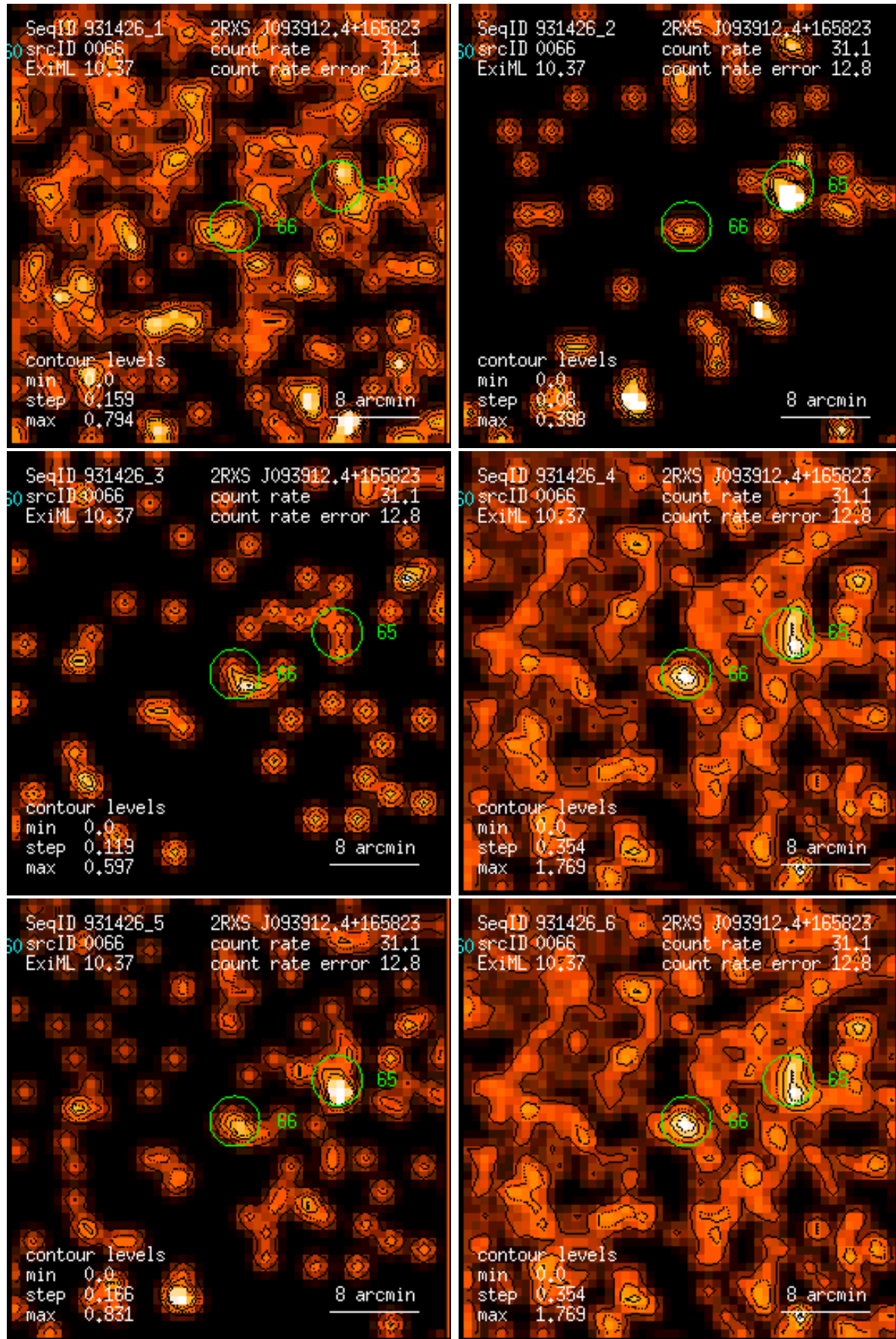
Figure 66: RASS 931426: detection 0066: band rate images, Gaussian filter: (1) PSPC channels 11 – 41, (2) 52 – 90, (3) 91 – 201, (4) 11 – 235, (5) 52 – 201, (6) 11 – 201. Broad band rates in counts/ks. Band rate contour levels in counts/ks/arcmin 2 .
