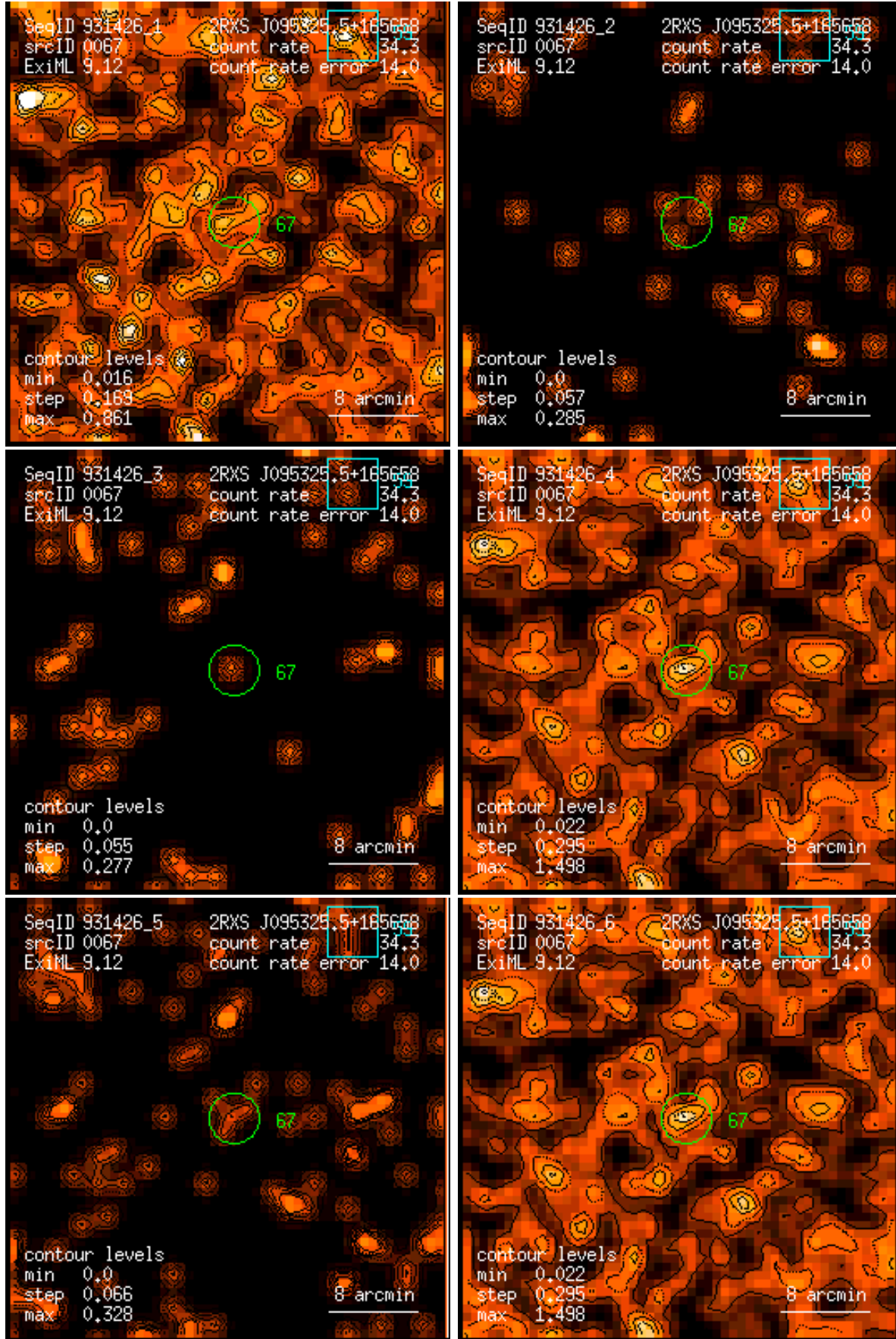
Figure 67: RASS 931426: detection 0067: band rate images, Gaussian filter: (1) PSPC channels 11 – 41, (2) 52 – 90, (3) 91 – 201, (4) 11 – 235, (5) 52 – 201, (6) 11 – 201. Broad band rates in counts/ks. Band rate contour levels in counts/ks/arcmin 2 .
