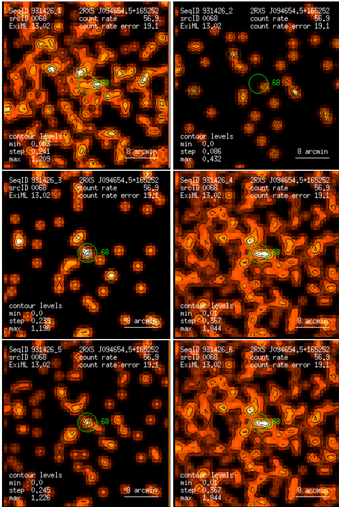
Figure 68: RASS 931426: detection 0068: band rate images, Gaussian filter: (1) PSPC channels 11 – 41, (2) 52 – 90, (3) 91 – 201, (4) 11 – 235, (5) 52 – 201, (6) 11 – 201. Broad band rates in counts/ks. Band rate contour levels in counts/ks/arcmin 2 .
