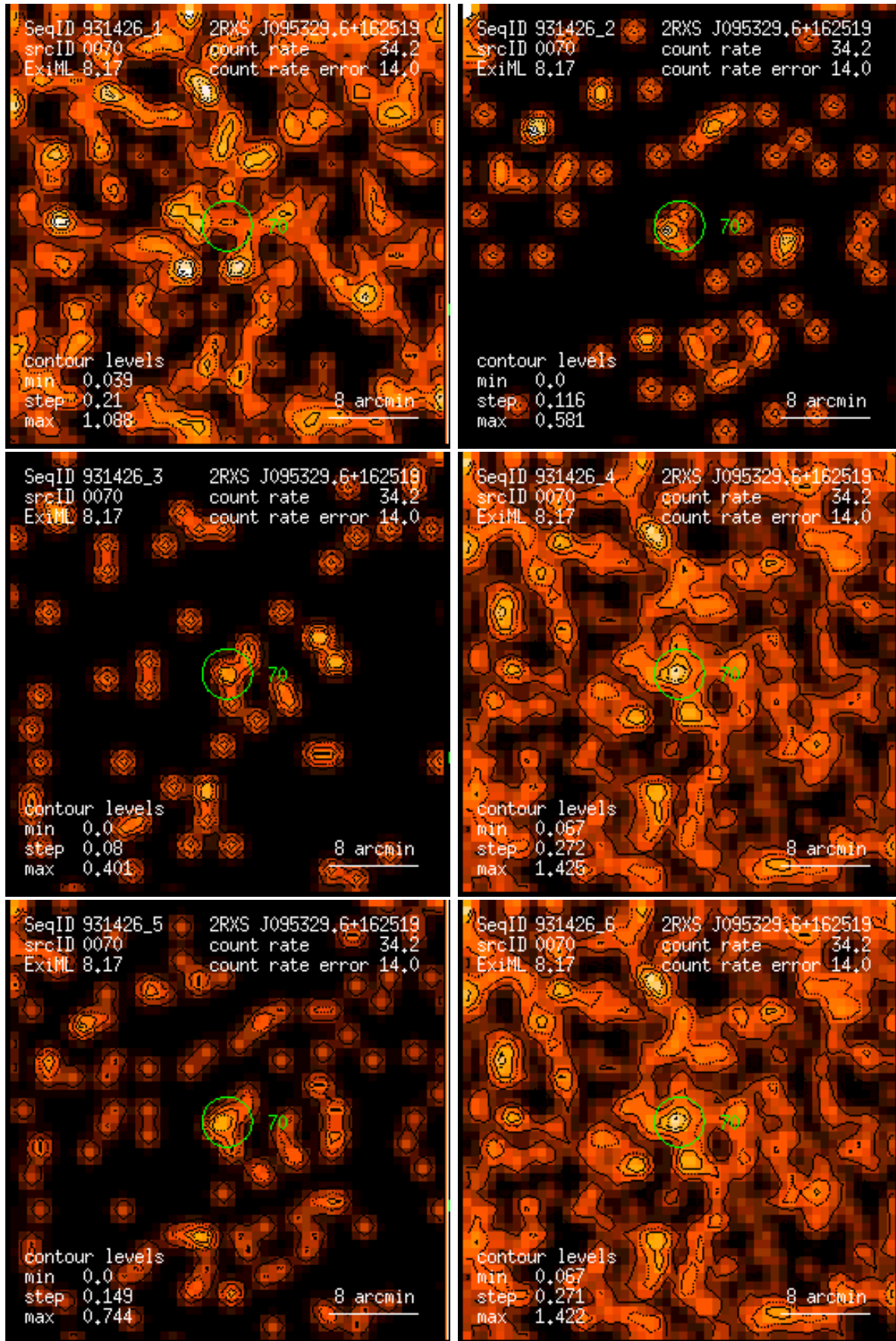
Figure 70: RASS 931426: detection 0070: band rate images, Gaussian filter: (1) PSPC channels 11 – 41, (2) 52 – 90, (3) 91 – 201, (4) 11 – 235, (5) 52 – 201, (6) 11 – 201. Broad band rates in counts/ks. Band rate contour levels in counts/ks/arcmin 2 .
