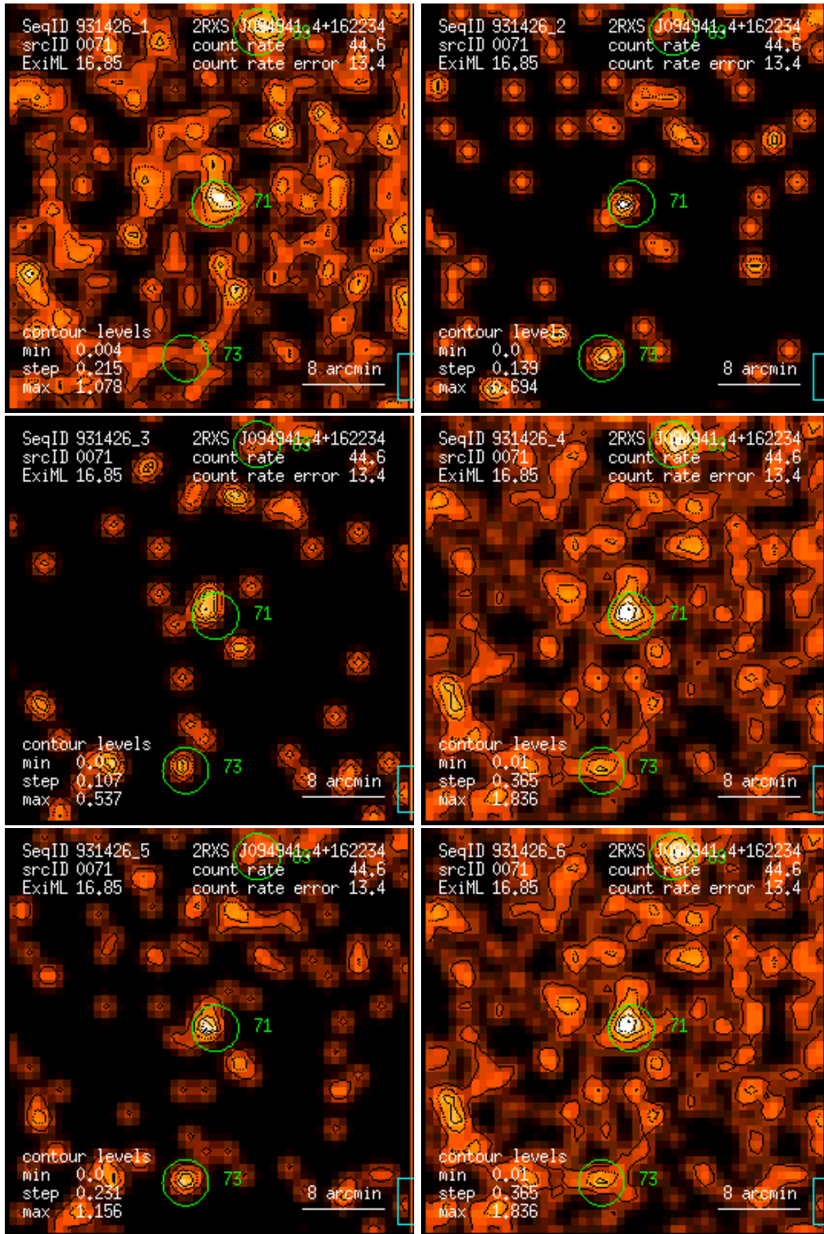
Figure 71: RASS 931426: detection 0071: band rate images, Gaussian filter: (1) PSPC channels 11 – 41, (2) 52 – 90, (3) 91 – 201, (4) 11 – 235, (5) 52 – 201, (6) 11 – 201. Broad band rates in counts/ks. Band rate contour levels in counts/ks/arcmin 2 .
