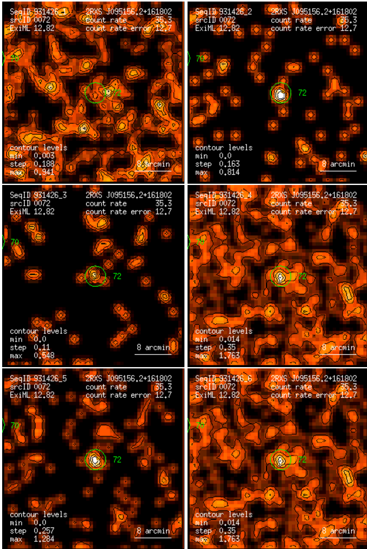
Figure 72: RASS 931426: detection 0072: band rate images, Gaussian filter: (1) PSPC channels 11 – 41, (2) 52 – 90, (3) 91 – 201, (4) 11 – 235, (5) 52 – 201, (6) 11 – 201. Broad band rates in counts/ks. Band rate contour levels in counts/ks/arcmin 2 .
