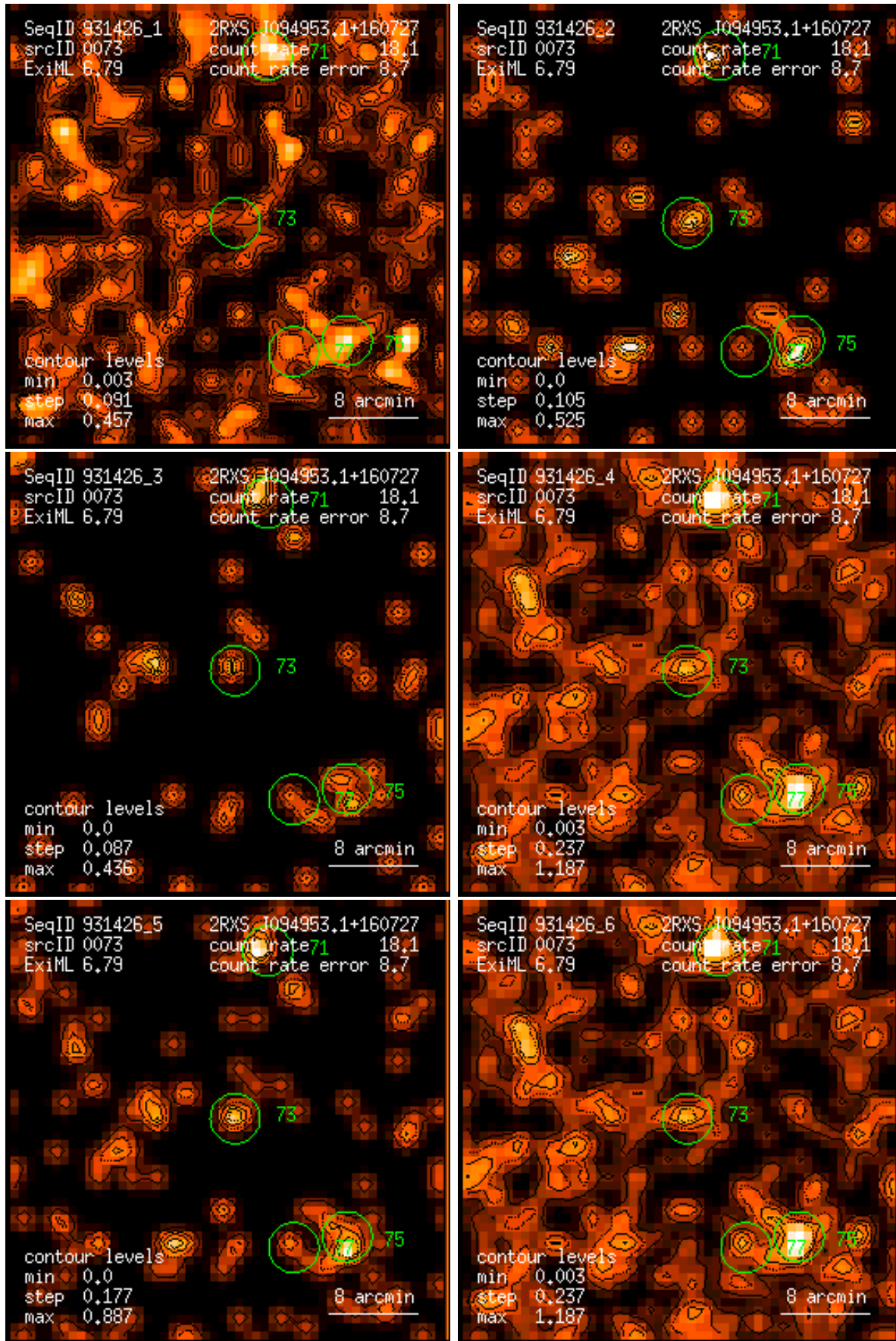
Figure 73: RASS 931426: detection 0073: band rate images, Gaussian filter: (1) PSPC channels 11 – 41, (2) 52 – 90, (3) 91 – 201, (4) 11 – 235, (5) 52 – 201, (6) 11 – 201. Broad band rates in counts/ks. Band rate contour levels in counts/ks/arcmin 2 .
