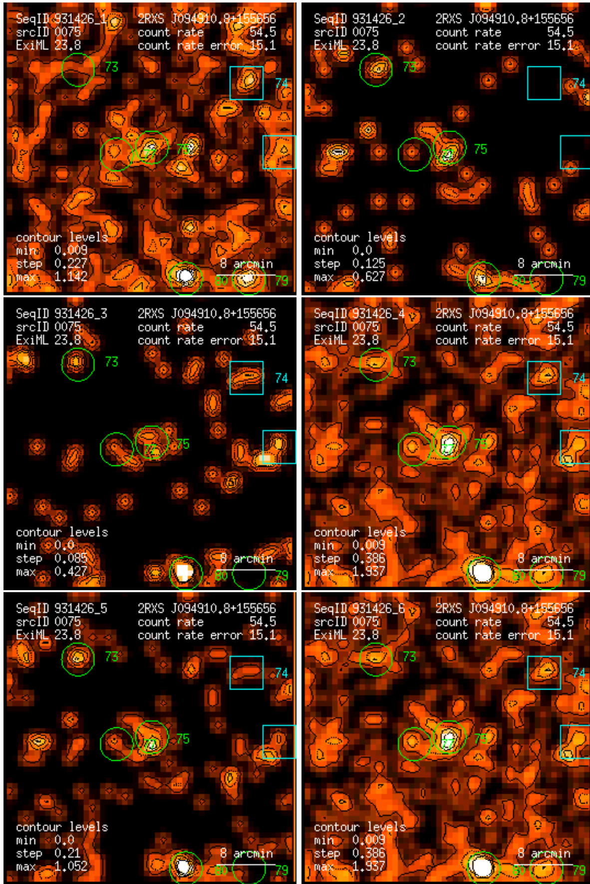
Figure 75: RASS 931426: detection 0075: band rate images, Gaussian filter: (1) PSPC channels 11 – 41, (2) 52 – 90, (3) 91 – 201, (4) 11 – 235, (5) 52 – 201, (6) 11 – 201. Broad band rates in counts/ks. Band rate contour levels in counts/ks/arcmin 2 .
