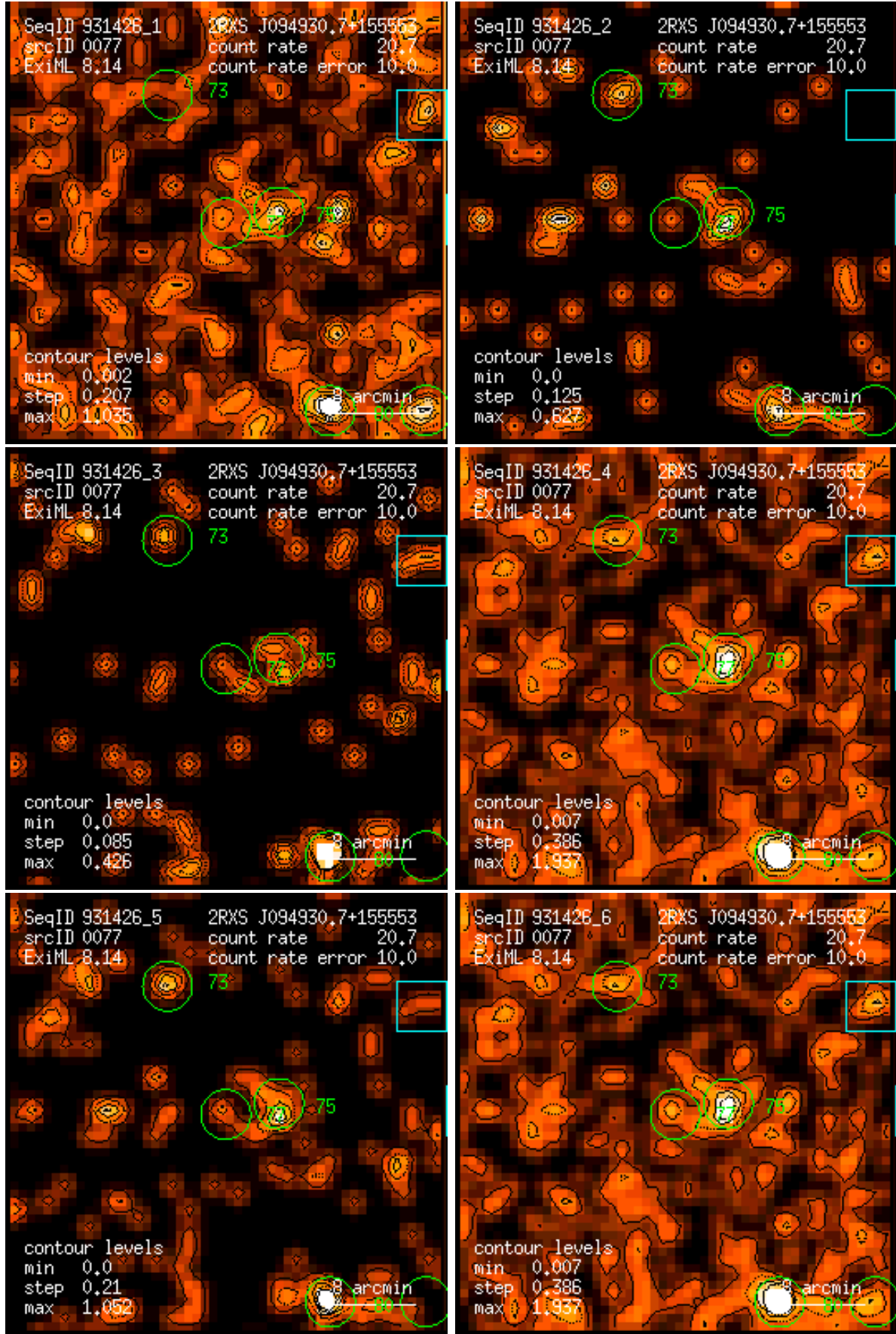
Figure 77: RASS 931426: detection 0077: band rate images, Gaussian filter: (1) PSPC channels 11 – 41, (2) 52 – 90, (3) 91 – 201, (4) 11 – 235, (5) 52 – 201, (6) 11 – 201. Broad band rates in counts/ks. Band rate contour levels in counts/ks/arcmin 2 .
