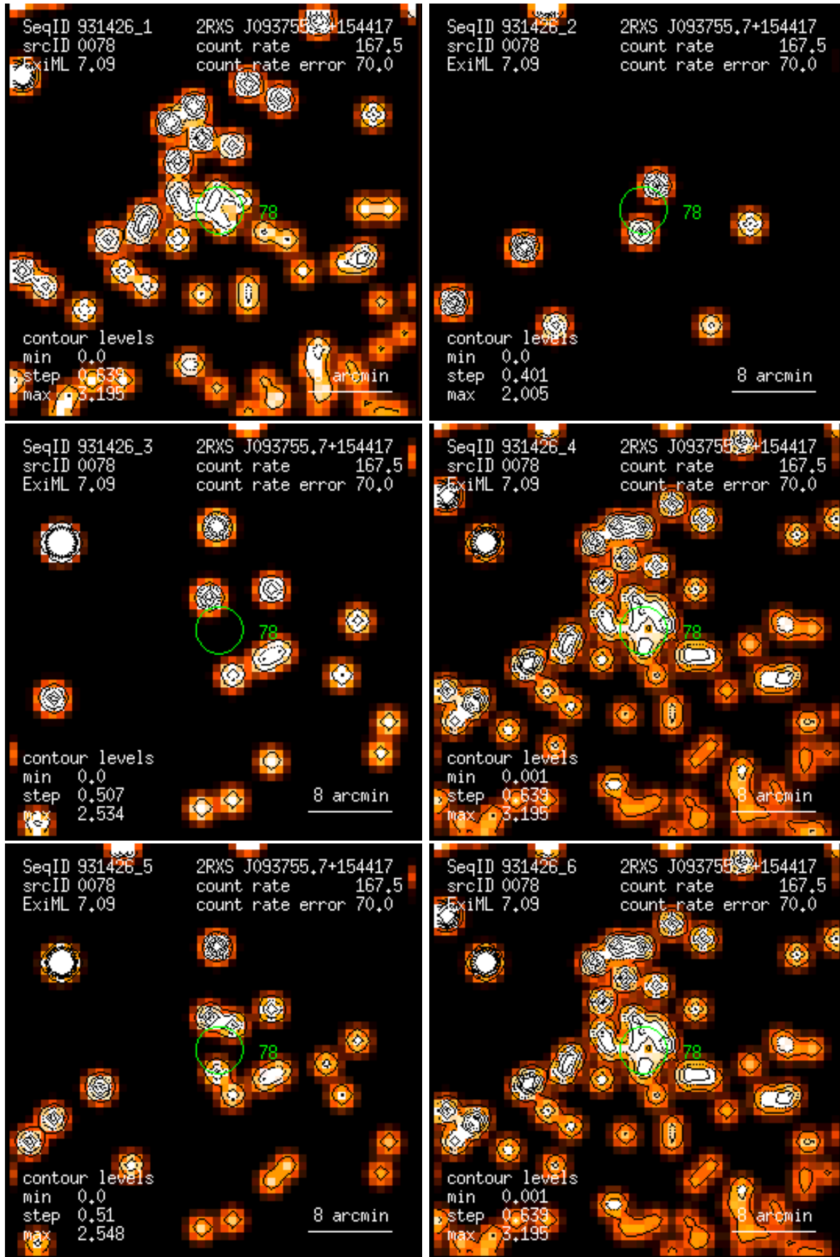
Figure 78: RASS 931426: detection 0078: band rate images, Gaussian filter: (1) PSPC channels 11 – 41, (2) 52 – 90, (3) 91 – 201, (4) 11 – 235, (5) 52 – 201, (6) 11 – 201. Broad band rates in counts/ks. Band rate contour levels in counts/ks/arcmin 2 .
