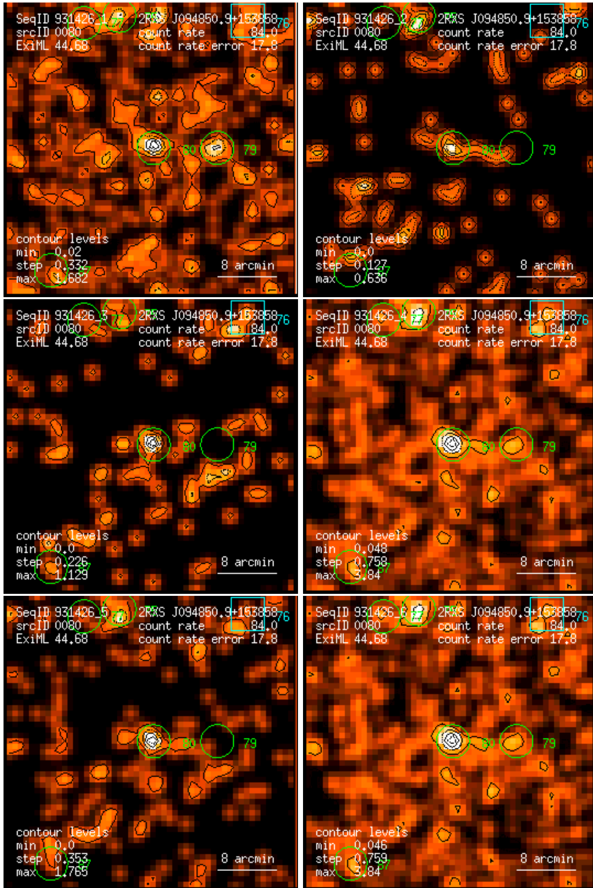
Figure 80: RASS 931426: detection 0080: band rate images, Gaussian filter: (1) PSPC channels 11 – 41, (2) 52 – 90, (3) 91 – 201, (4) 11 – 235, (5) 52 – 201, (6) 11 – 201. Broad band rates in counts/ks. Band rate contour levels in counts/ks/arcmin 2 .
