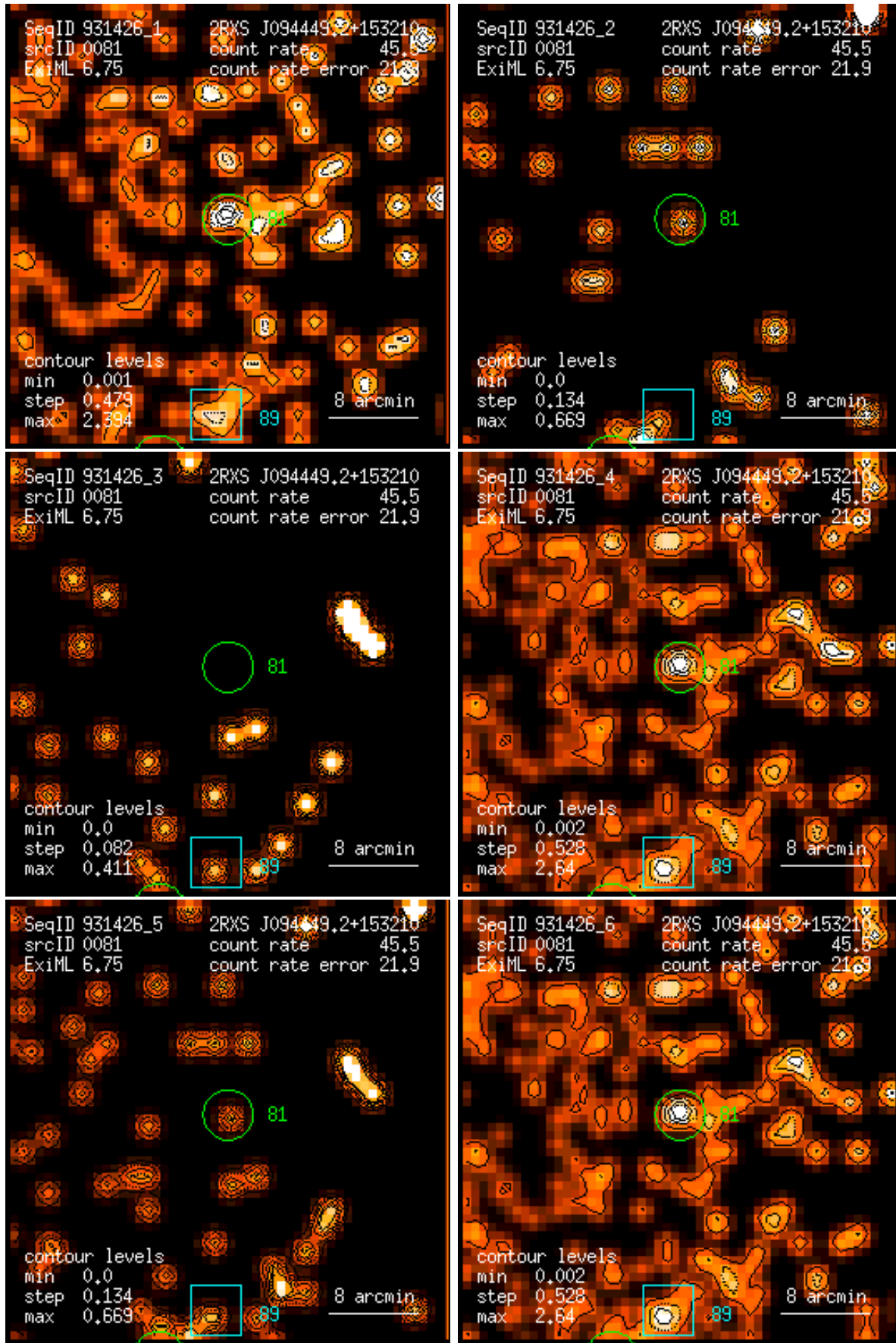
Figure 81: RASS 931426: detection 0081: band rate images, Gaussian filter: (1) PSPC channels 11 – 41, (2) 52 – 90, (3) 91 – 201, (4) 11 – 235, (5) 52 – 201, (6) 11 – 201. Broad band rates in counts/ks. Band rate contour levels in counts/ks/arcmin 2 .
