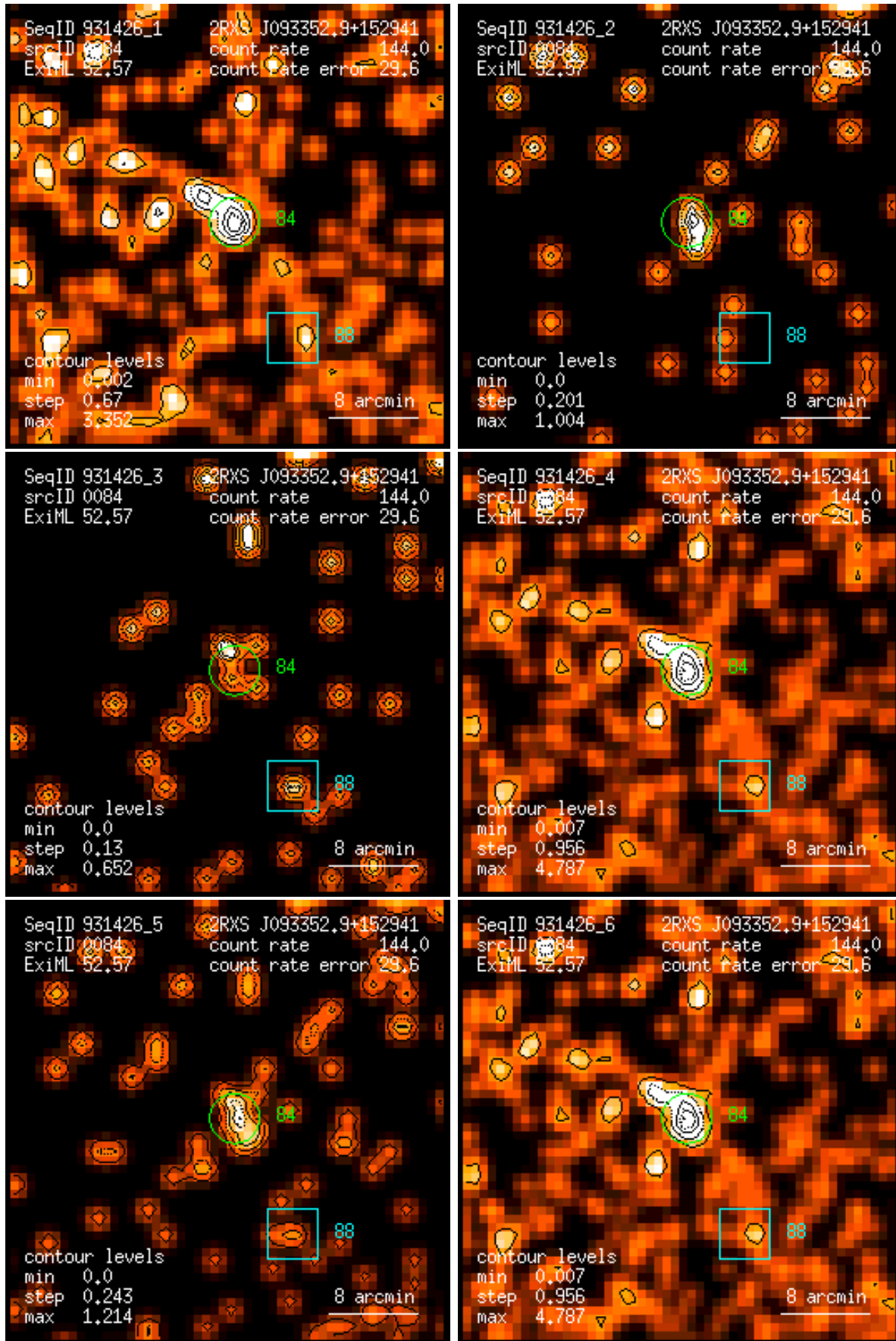
Figure 84: RASS 931426: detection 0084: band rate images, Gaussian filter: (1) PSPC channels 11 – 41, (2) 52 – 90, (3) 91 – 201, (4) 11 – 235, (5) 52 – 201, (6) 11 – 201. Broad band rates in counts/ks. Band rate contour levels in counts/ks/arcmin 2 .
