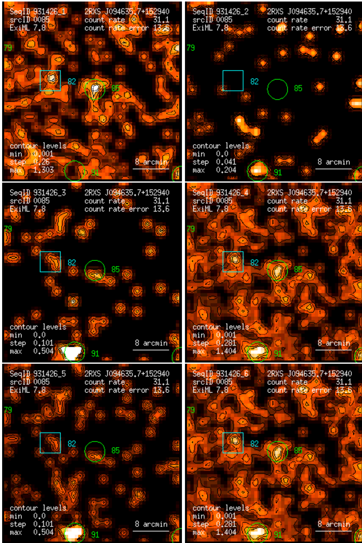
Figure 85: RASS 931426: detection 0085: band rate images, Gaussian filter: (1) PSPC channels 11 – 41, (2) 52 – 90, (3) 91 – 201, (4) 11 – 235, (5) 52 – 201, (6) 11 – 201. Broad band rates in counts/ks. Band rate contour levels in counts/ks/arcmin 2 .
