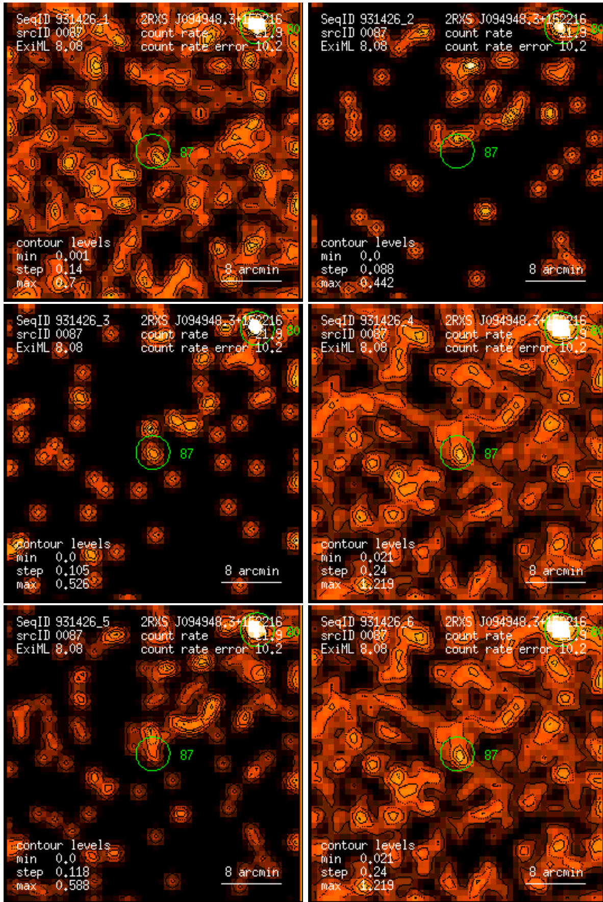
Figure 87: RASS 931426: detection 0087: band rate images, Gaussian filter: (1) PSPC channels 11 – 41, (2) 52 – 90, (3) 91 – 201, (4) 11 – 235, (5) 52 – 201, (6) 11 – 201. Broad band rates in counts/ks. Band rate contour levels in counts/ks/arcmin 2 .
