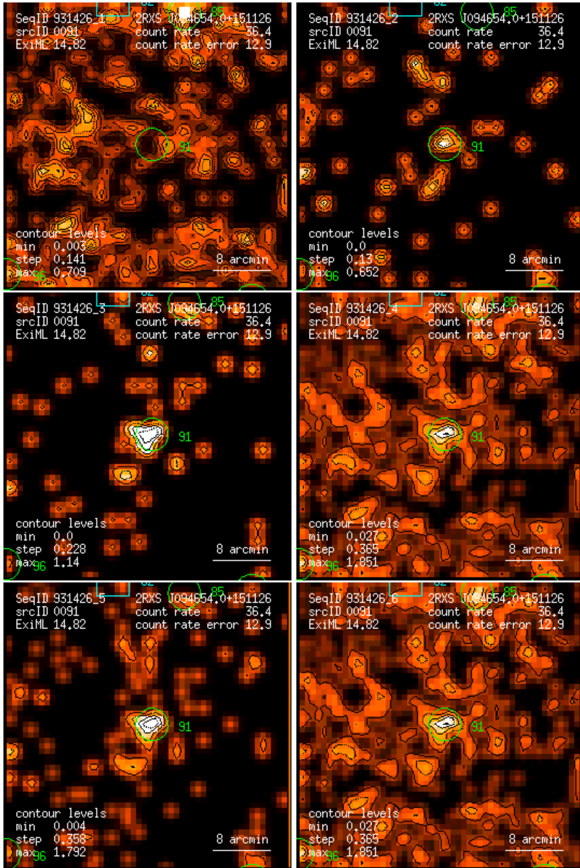
Figure 91: RASS 931426: detection 0091: band rate images, Gaussian filter: (1) PSPC channels 11 – 41, (2) 52 – 90, (3) 91 – 201, (4) 11 – 235, (5) 52 – 201, (6) 11 – 201. Broad band rates in counts/ks. Band rate contour levels in counts/ks/arcmin 2 .
