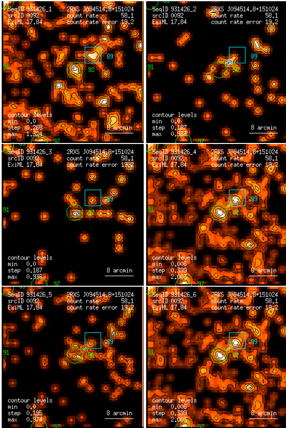
Figure 92: RASS 931426: detection 0092: band rate images, Gaussian filter: (1) PSPC channels 11 – 41, (2) 52 – 90, (3) 91 – 201, (4) 11 – 235, (5) 52 – 201, (6) 11 – 201. Broad band rates in counts/ks. Band rate contour levels in counts/ks/arcmin 2 .
