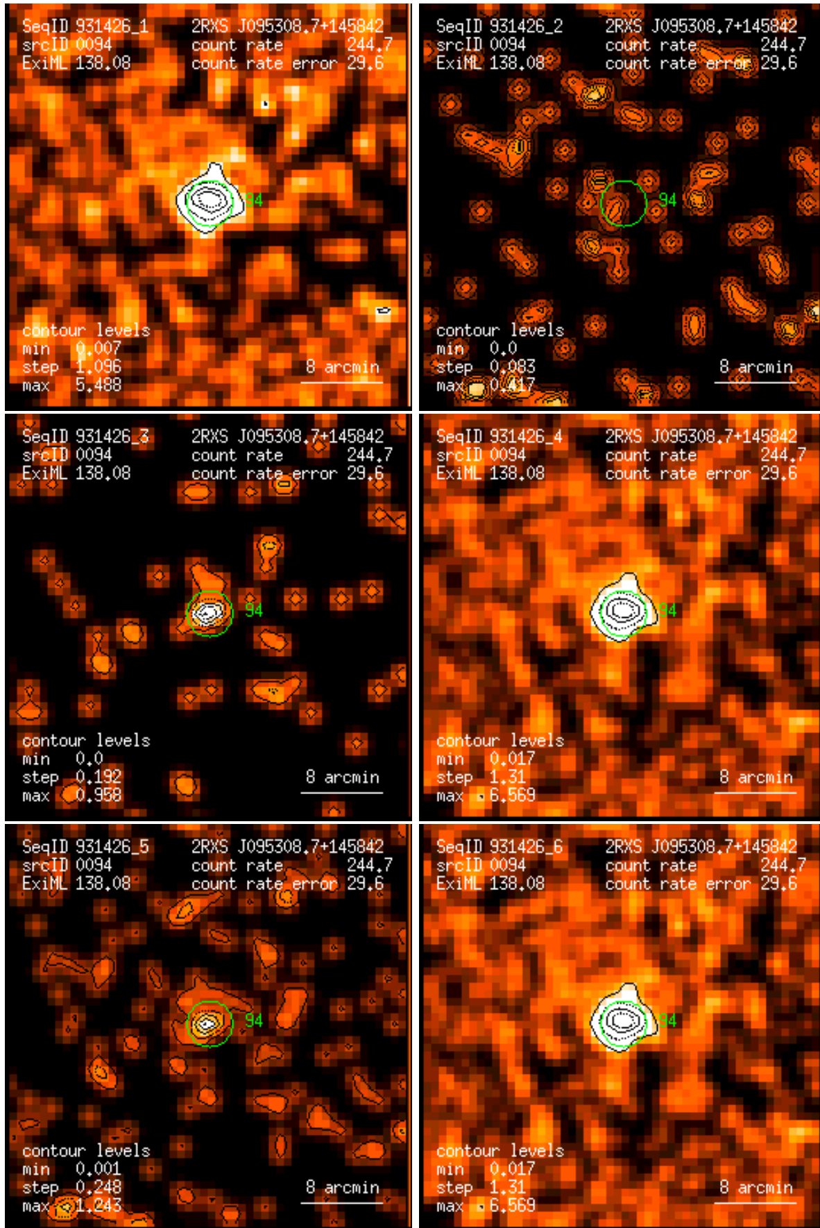
Figure 94: RASS 931426: detection 0094: band rate images, Gaussian filter: (1) PSPC channels 11 – 41, (2) 52 – 90, (3) 91 – 201, (4) 11 – 235, (5) 52 – 201, (6) 11 – 201. Broad band rates in counts/ks. Band rate contour levels in counts/ks/arcmin 2 .
