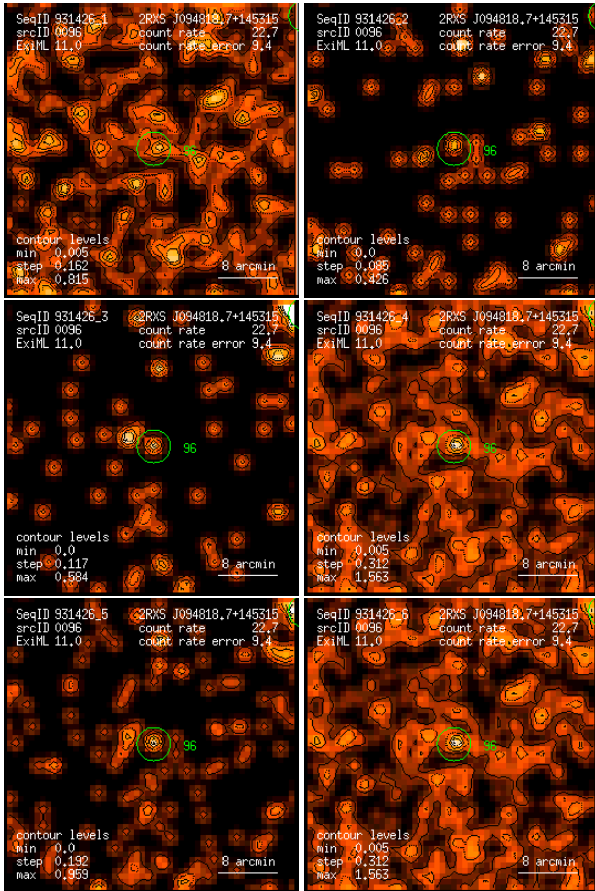
Figure 96: RASS 931426: detection 0096: band rate images, Gaussian filter: (1) PSPC channels 11 – 41, (2) 52 – 90, (3) 91 – 201, (4) 11 – 235, (5) 52 – 201, (6) 11 – 201. Broad band rates in counts/ks. Band rate contour levels in counts/ks/arcmin 2 .
