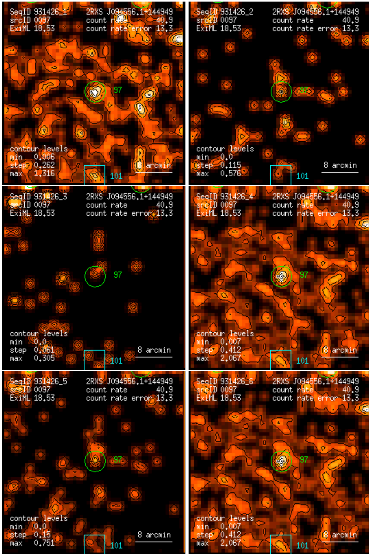
Figure 97: RASS 931426: detection 0097: band rate images, Gaussian filter: (1) PSPC channels 11 – 41, (2) 52 – 90, (3) 91 – 201, (4) 11 – 235, (5) 52 – 201, (6) 11 – 201. Broad band rates in counts/ks. Band rate contour levels in counts/ks/arcmin 2 .
