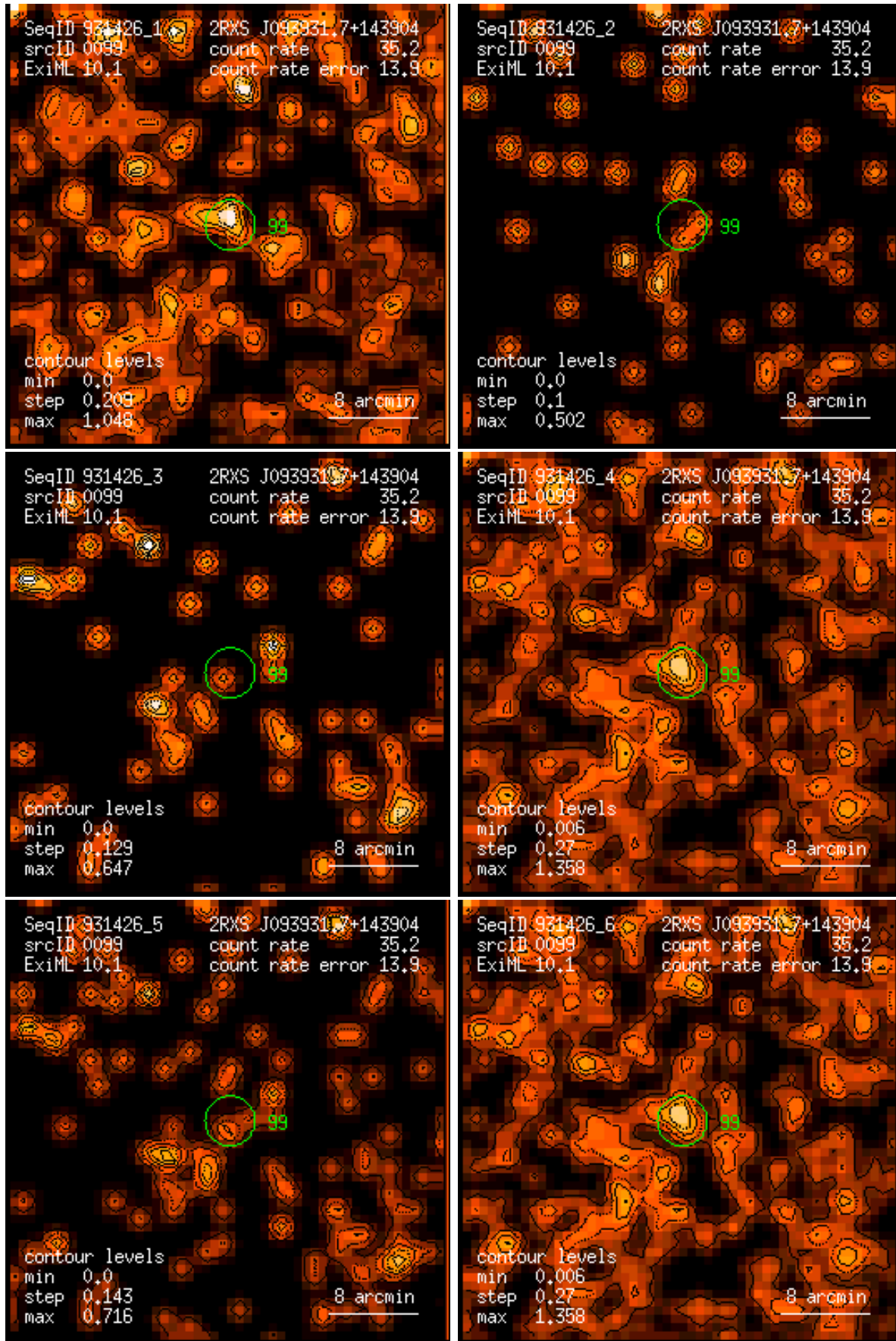
Figure 99: RASS 931426: detection 0099: band rate images, Gaussian filter: (1) PSPC channels 11 – 41, (2) 52 – 90, (3) 91 – 201, (4) 11 – 235, (5) 52 – 201, (6) 11 – 201. Broad band rates in counts/ks. Band rate contour levels in counts/ks/arcmin 2 .
