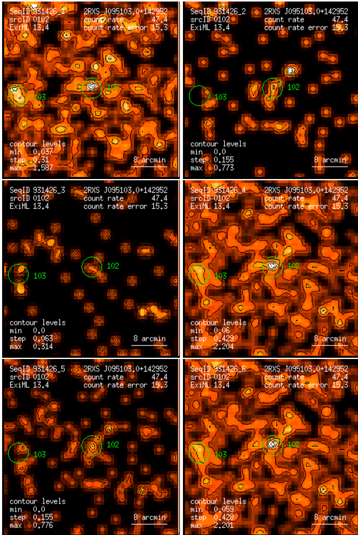
Figure 102: RASS 931426: detection 0102: band rate images, Gaussian filter: (1) PSPC channels 11 – 41, (2) 52 – 90, (3) 91 – 201, (4) 11 – 235, (5) 52 – 201, (6) 11 – 201. Broad band rates in counts/ks. Band rate contour levels in counts/ks/arcmin 2 .
