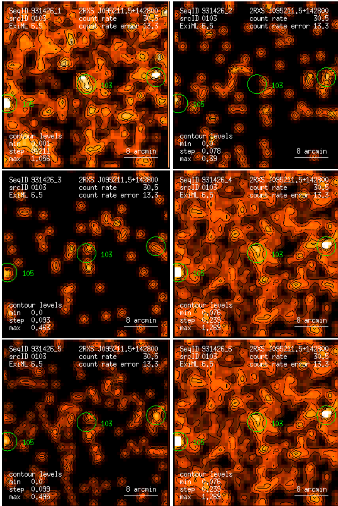
Figure 103: RASS 931426: detection 0103: band rate images, Gaussian filter: (1) PSPC channels 11 – 41, (2) 52 – 90, (3) 91 – 201, (4) 11 – 235, (5) 52 – 201, (6) 11 – 201. Broad band rates in counts/ks. Band rate contour levels in counts/ks/arcmin 2 .
