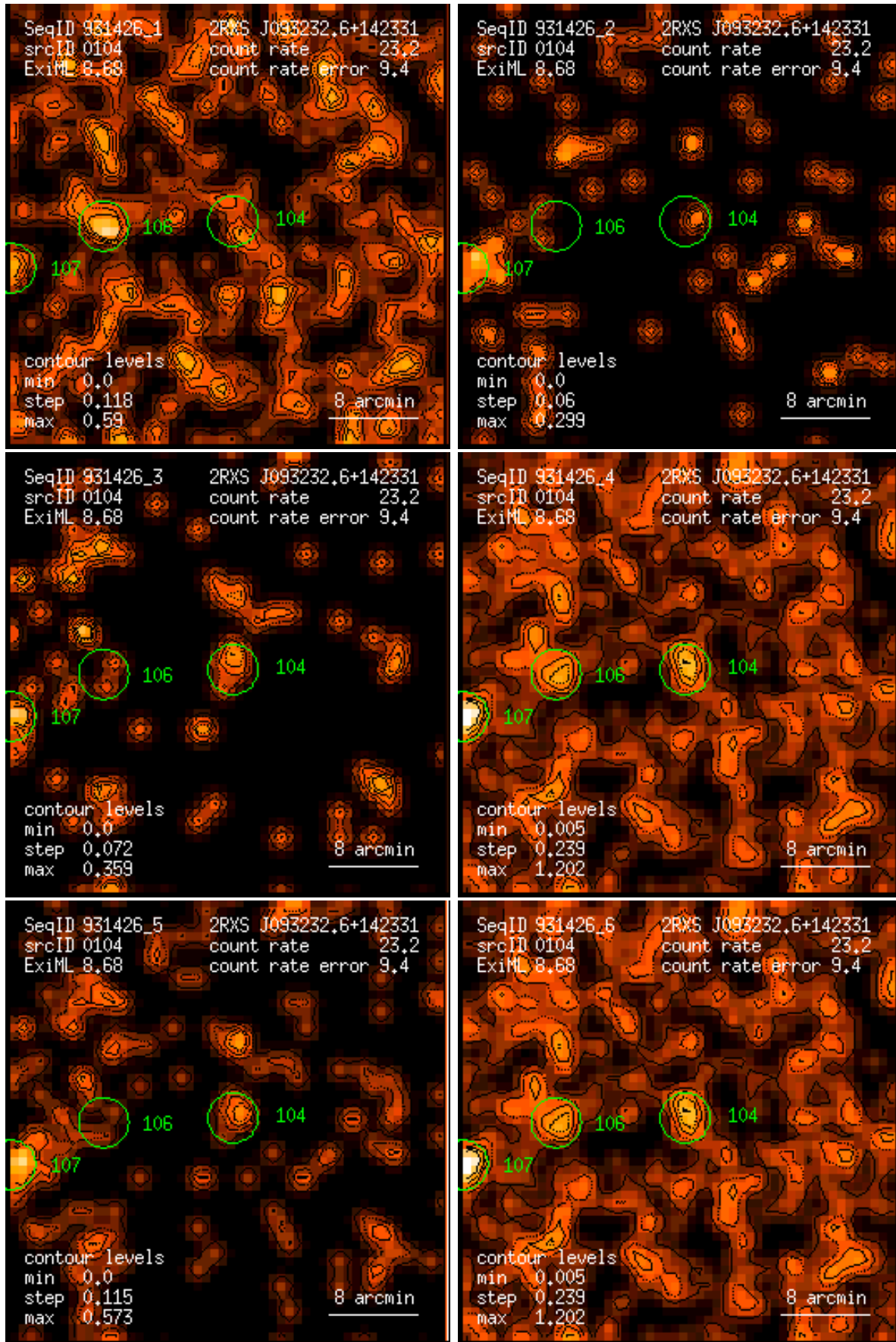
Figure 104: RASS 931426: detection 0104: band rate images, Gaussian filter: (1) PSPC channels 11 – 41, (2) 52 – 90, (3) 91 – 201, (4) 11 – 235, (5) 52 – 201, (6) 11 – 201. Broad band rates in counts/ks. Band rate contour levels in counts/ks/arcmin 2 .
