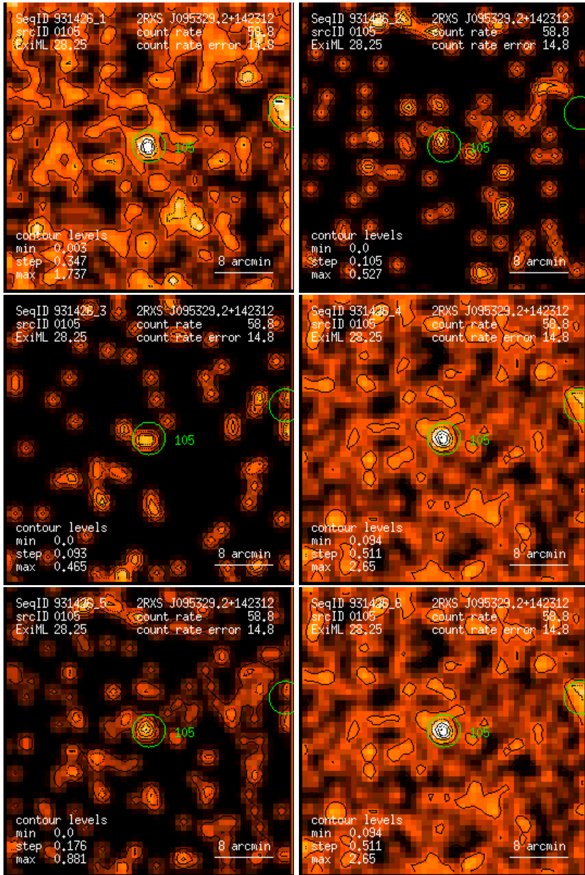
Figure 105: RASS 931426: detection 0105: band rate images, Gaussian filter: (1) PSPC channels 11 – 41, (2) 52 – 90, (3) 91 – 201, (4) 11 – 235, (5) 52 – 201, (6) 11 – 201. Broad band rates in counts/ks. Band rate contour levels in counts/ks/arcmin 2 .
