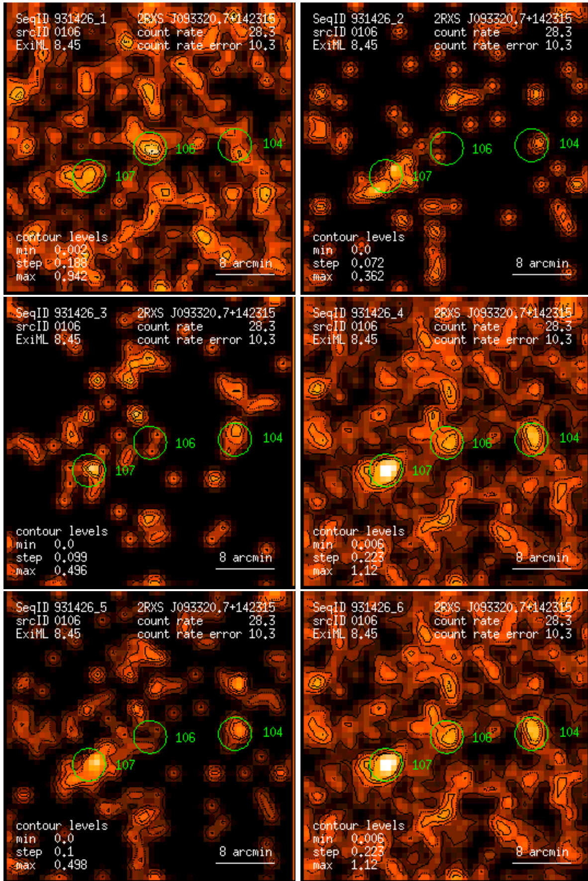
Figure 106: RASS 931426: detection 0106: band rate images, Gaussian filter: (1) PSPC channels 11 – 41, (2) 52 – 90, (3) 91 – 201, (4) 11 – 235, (5) 52 – 201, (6) 11 – 201. Broad band rates in counts/ks. Band rate contour levels in counts/ks/arcmin 2 .
