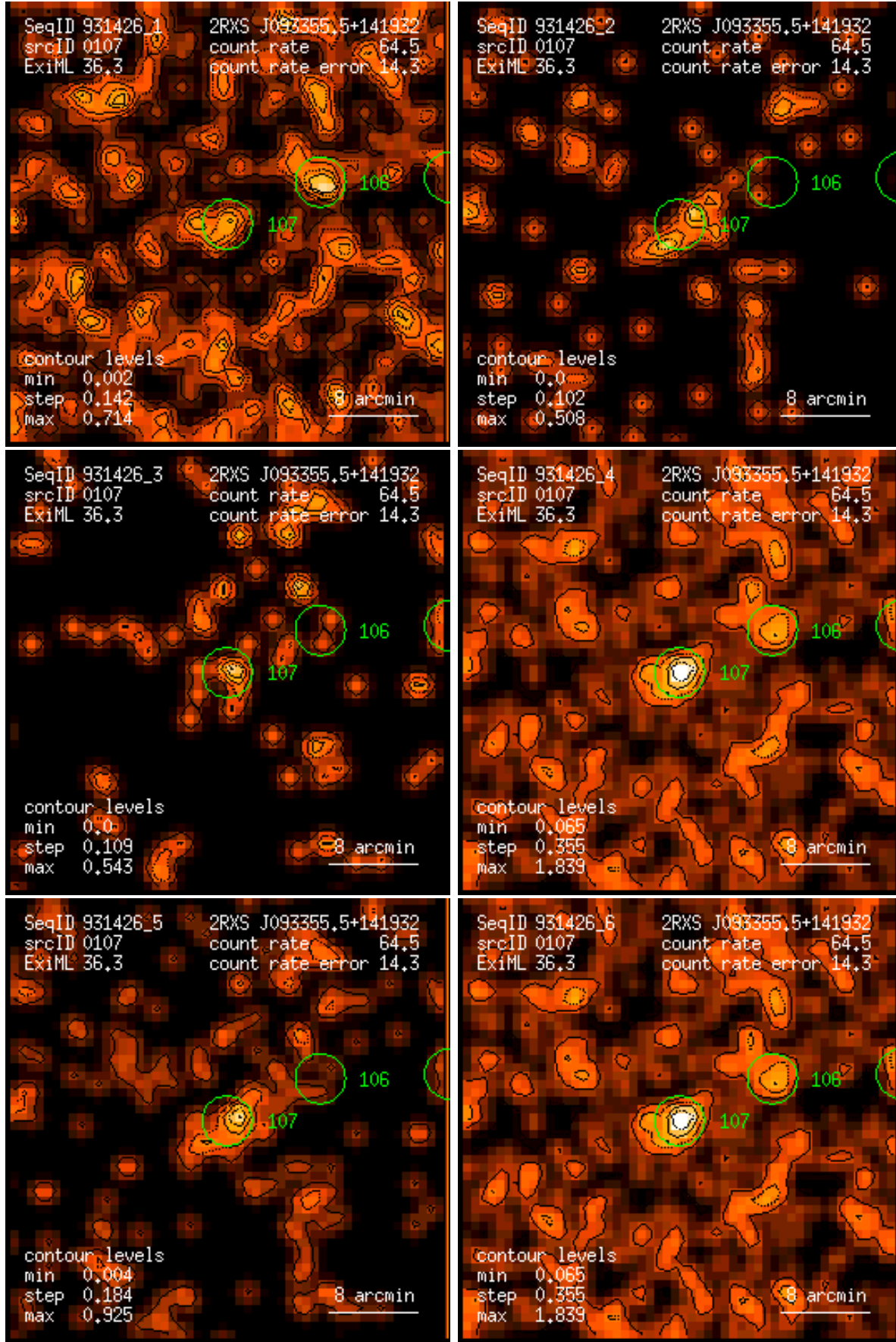
Figure 107: RASS 931426: detection 0107: band rate images, Gaussian filter: (1) PSPC channels 11 – 41, (2) 52 – 90, (3) 91 – 201, (4) 11 – 235, (5) 52 – 201, (6) 11 – 201. Broad band rates in counts/ks. Band rate contour levels in counts/ks/arcmin 2 .
