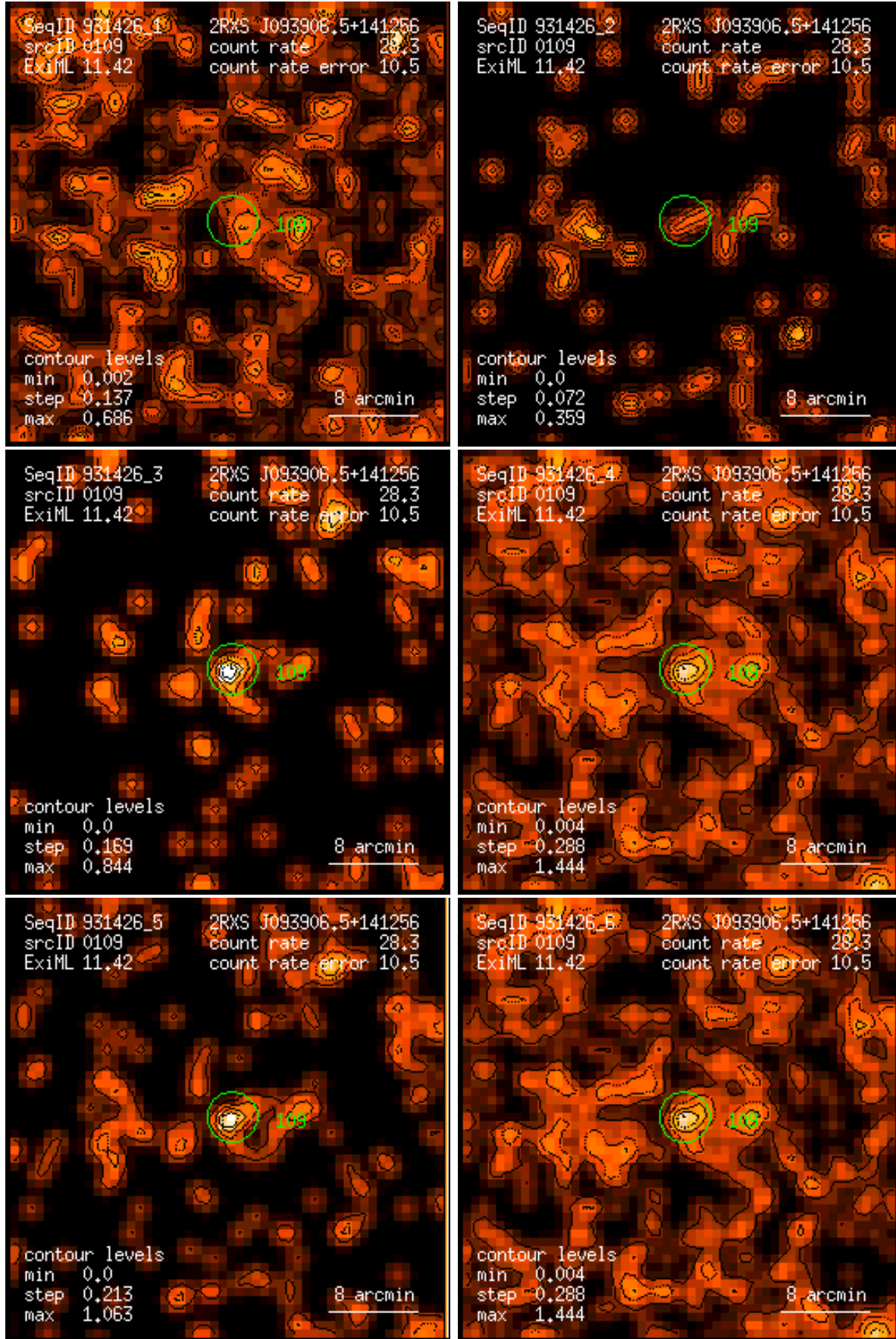
Figure 109: RASS 931426: detection 0109: band rate images, Gaussian filter: (1) PSPC channels 11 – 41, (2) 52 – 90, (3) 91 – 201, (4) 11 – 235, (5) 52 – 201, (6) 11 – 201. Broad band rates in counts/ks. Band rate contour levels in counts/ks/arcmin 2 .
