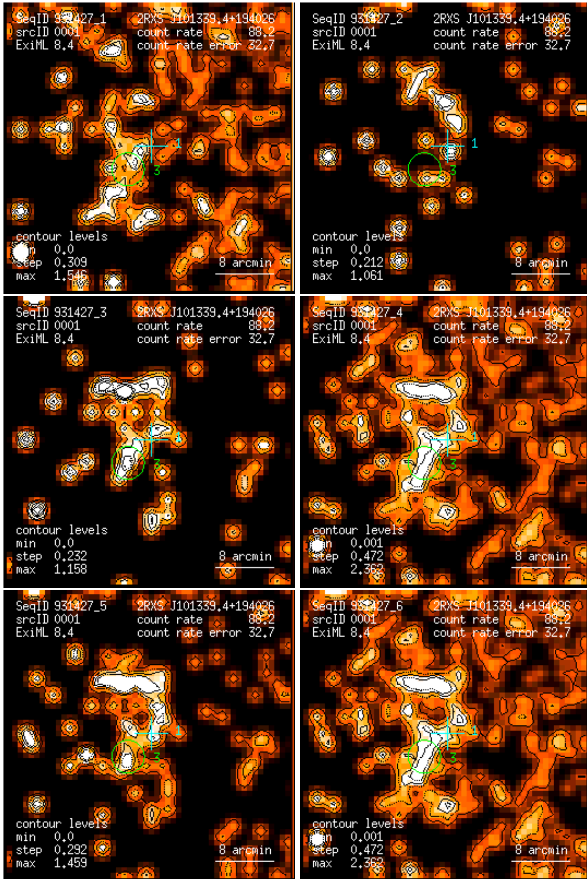
Figure 1: RASS 931427: detection 0001: band rate images, Gaussian filter: (1) PSPC channels 11 – 41, (2) 52 – 90, (3) 91 – 201, (4) 11 – 235, (5) 52 – 201, (6) 11 – 201. Broad band rates in counts/ks. Band rate contour levels in counts/ks/arcmin 2 .
