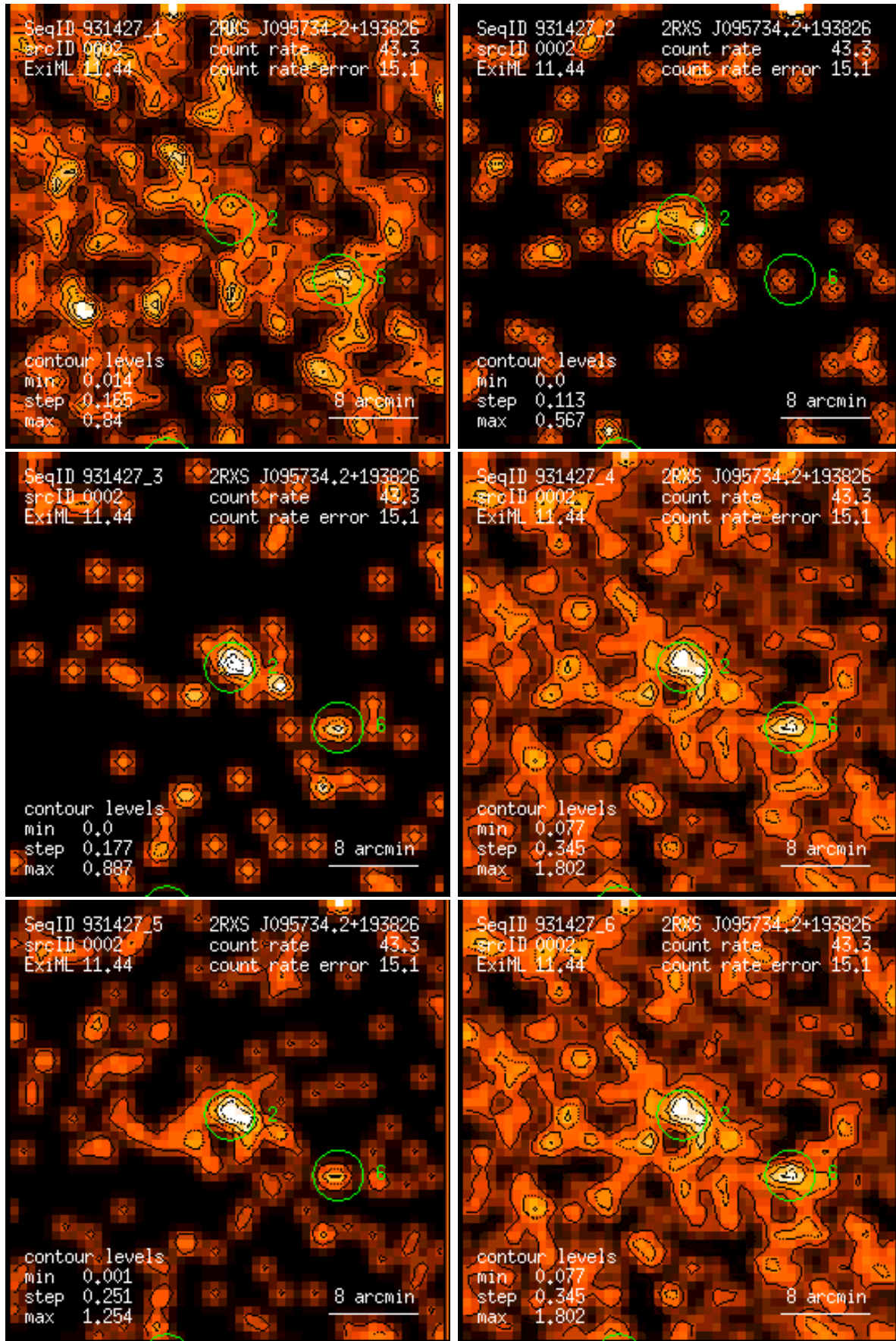
Figure 2: RASS 931427: detection 0002: band rate images, Gaussian filter: (1) PSPC channels 11 – 41, (2) 52 – 90, (3) 91 – 201, (4) 11 – 235, (5) 52 – 201, (6) 11 – 201. Broad band rates in counts/ks. Band rate contour levels in counts/ks/arcmin 2 .
