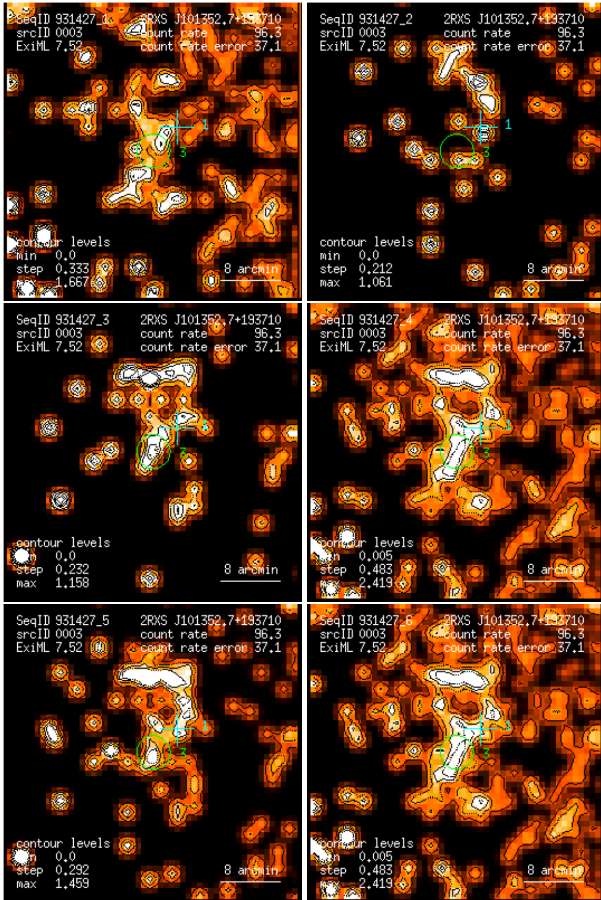
Figure 3: RASS 931427: detection 0003: band rate images, Gaussian filter: (1) PSPC channels 11 – 41, (2) 52 – 90, (3) 91 – 201, (4) 11 – 235, (5) 52 – 201, (6) 11 – 201. Broad band rates in counts/ks. Band rate contour levels in counts/ks/arcmin 2 .
