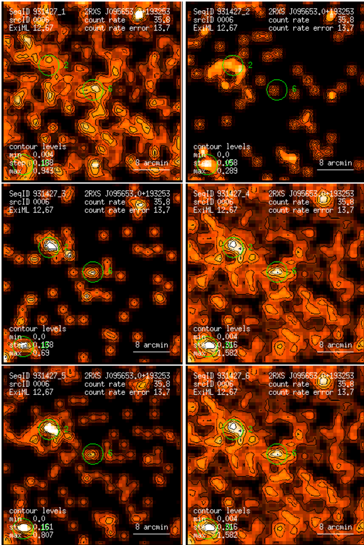
Figure 6: RASS 931427: detection 0006: band rate images, Gaussian filter: (1) PSPC channels 11 – 41, (2) 52 – 90, (3) 91 – 201, (4) 11 – 235, (5) 52 – 201, (6) 11 – 201. Broad band rates in counts/ks. Band rate contour levels in counts/ks/arcmin 2 .
