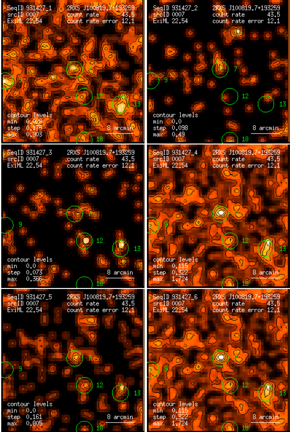
Figure 7: RASS 931427: detection 0007: band rate images, Gaussian filter: (1) PSPC channels 11 – 41, (2) 52 – 90, (3) 91 – 201, (4) 11 – 235, (5) 52 – 201, (6) 11 – 201. Broad band rates in counts/ks. Band rate contour levels in counts/ks/arcmin 2 .
