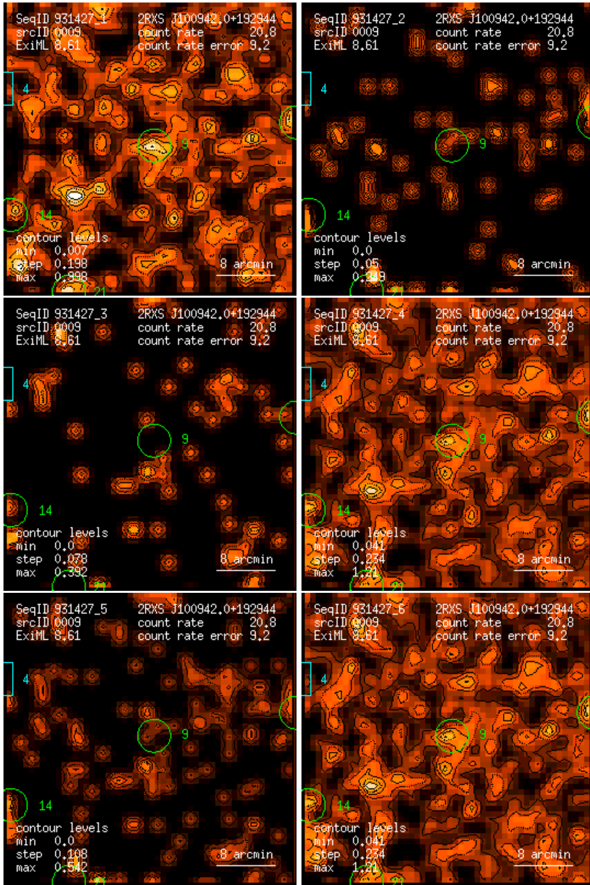
Figure 9: RASS 931427: detection 0009: band rate images, Gaussian filter: (1) PSPC channels 11 – 41, (2) 52 – 90, (3) 91 – 201, (4) 11 – 235, (5) 52 – 201, (6) 11 – 201. Broad band rates in counts/ks. Band rate contour levels in counts/ks/arcmin 2 .
