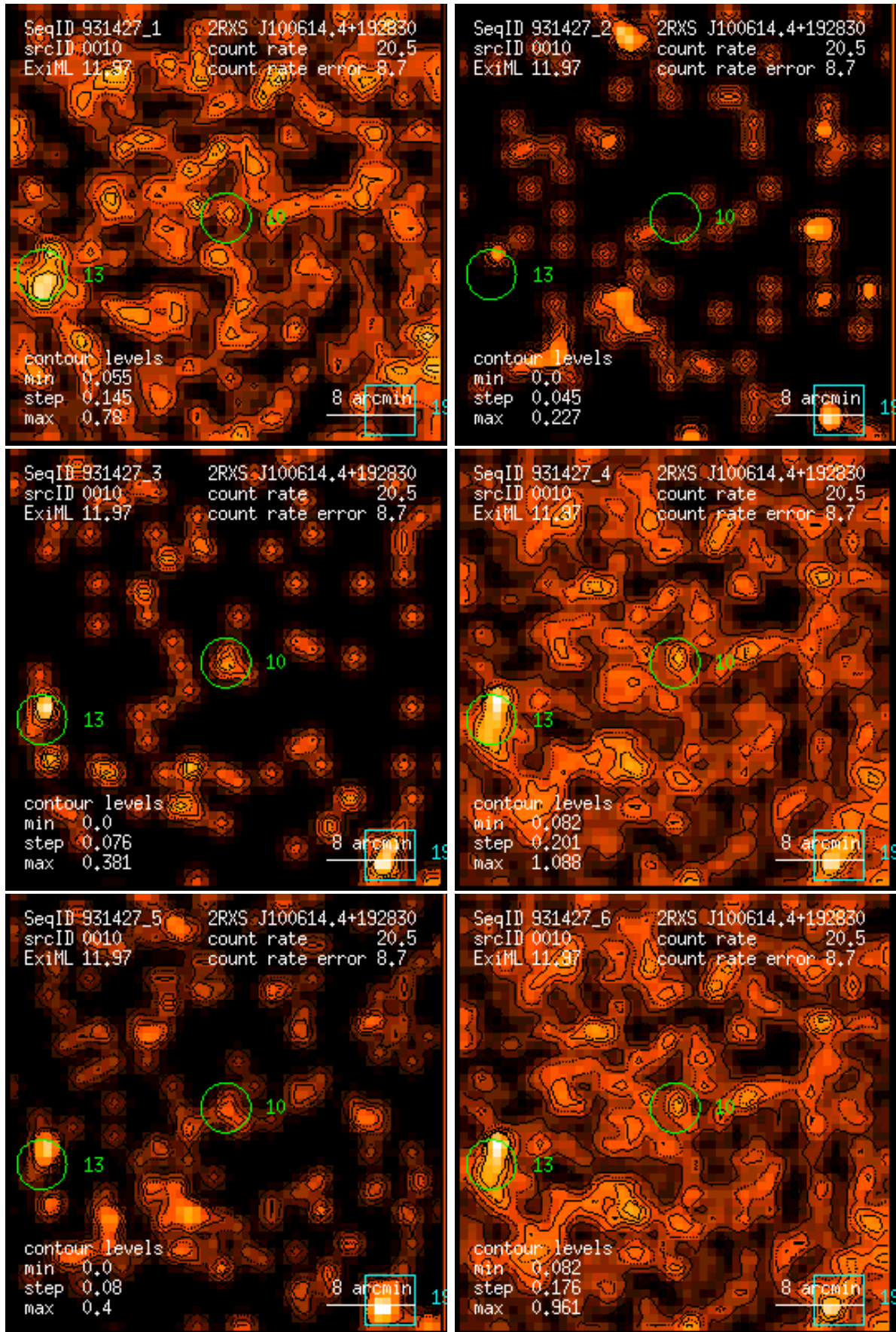
Figure 10: RASS 931427: detection 0010: band rate images, Gaussian filter: (1) PSPC channels 11 – 41, (2) 52 – 90, (3) 91 – 201, (4) 11 – 235, (5) 52 – 201, (6) 11 – 201. Broad band rates in counts/ks. Band rate contour levels in counts/ks/arcmin 2 .
