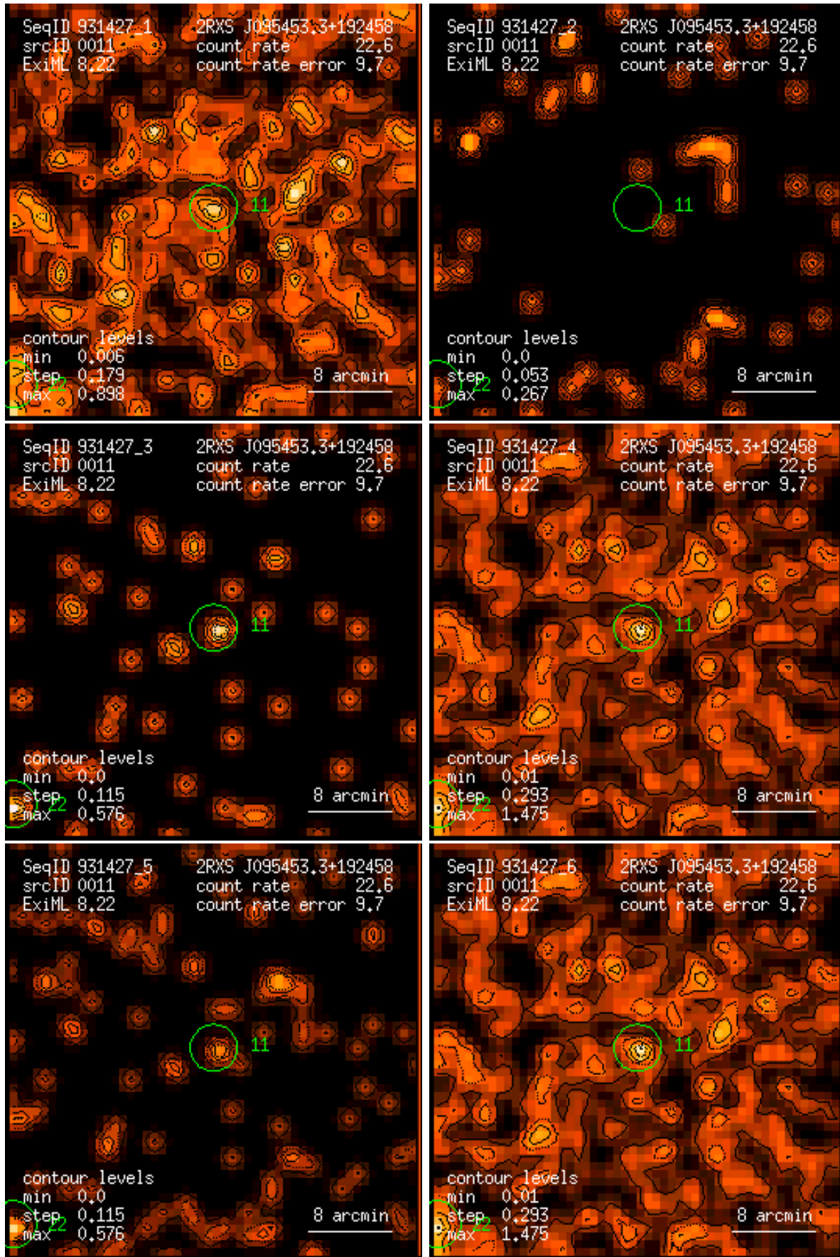
Figure 11: RASS 931427: detection 0011: band rate images, Gaussian filter: (1) PSPC channels 11 – 41, (2) 52 – 90, (3) 91 – 201, (4) 11 – 235, (5) 52 – 201, (6) 11 – 201. Broad band rates in counts/ks. Band rate contour levels in counts/ks/arcmin 2 .
