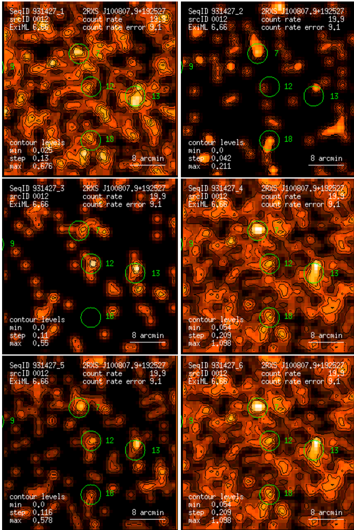
Figure 12: RASS 931427: detection 0012: band rate images, Gaussian filter: (1) PSPC channels 11 – 41, (2) 52 – 90, (3) 91 – 201, (4) 11 – 235, (5) 52 – 201, (6) 11 – 201. Broad band rates in counts/ks. Band rate contour levels in counts/ks/arcmin 2 .
