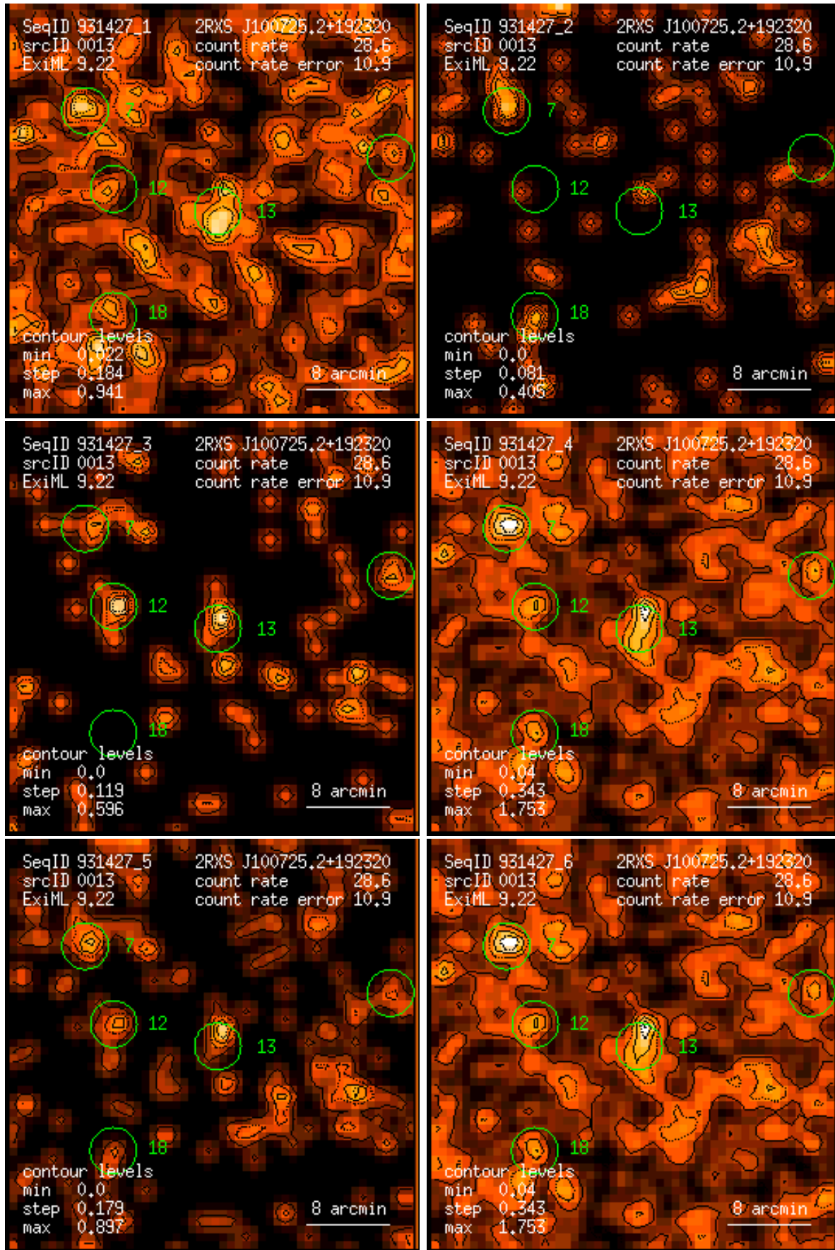
Figure 13: RASS 931427: detection 0013: band rate images, Gaussian filter: (1) PSPC channels 11 – 41, (2) 52 – 90, (3) 91 – 201, (4) 11 – 235, (5) 52 – 201, (6) 11 – 201. Broad band rates in counts/ks. Band rate contour levels in counts/ks/arcmin 2 .
