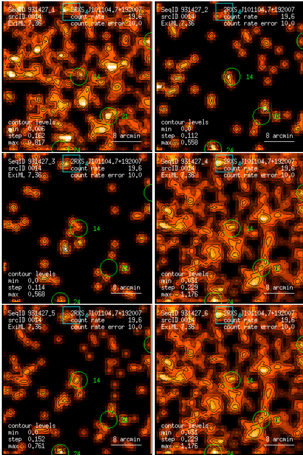
Figure 14: RASS 931427: detection 0014: band rate images, Gaussian filter: (1) PSPC channels 11 – 41, (2) 52 – 90, (3) 91 – 201, (4) 11 – 235, (5) 52 – 201, (6) 11 – 201. Broad band rates in counts/ks. Band rate contour levels in counts/ks/arcmin 2 .
