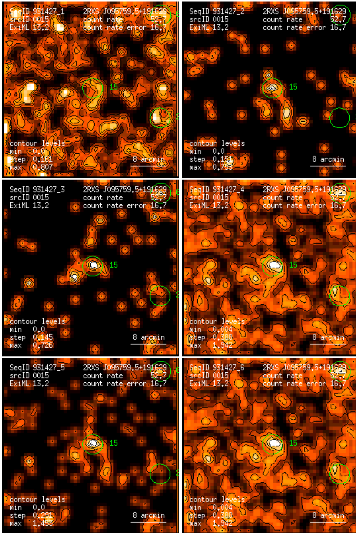
Figure 15: RASS 931427: detection 0015: band rate images, Gaussian filter: (1) PSPC channels 11 – 41, (2) 52 – 90, (3) 91 – 201, (4) 11 – 235, (5) 52 – 201, (6) 11 – 201. Broad band rates in counts/ks. Band rate contour levels in counts/ks/arcmin 2 .
