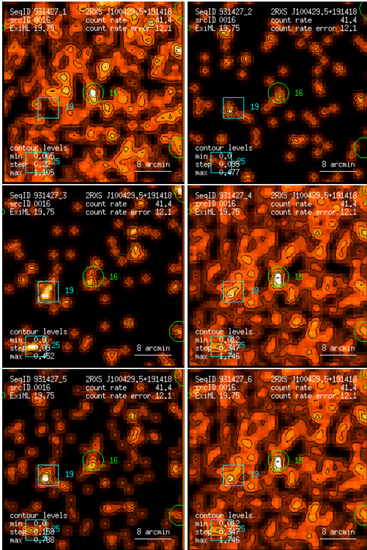
Figure 16: RASS 931427: detection 0016: band rate images, Gaussian filter: (1) PSPC channels 11 – 41, (2) 52 – 90, (3) 91 – 201, (4) 11 – 235, (5) 52 – 201, (6) 11 – 201. Broad band rates in counts/ks. Band rate contour levels in counts/ks/arcmin 2 .
