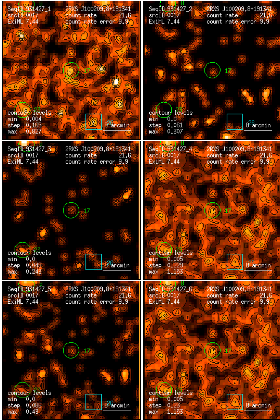
Figure 17: RASS 931427: detection 0017: band rate images, Gaussian filter: (1) PSPC channels 11 – 41, (2) 52 – 90, (3) 91 – 201, (4) 11 – 235, (5) 52 – 201, (6) 11 – 201. Broad band rates in counts/ks. Band rate contour levels in counts/ks/arcmin 2 .
