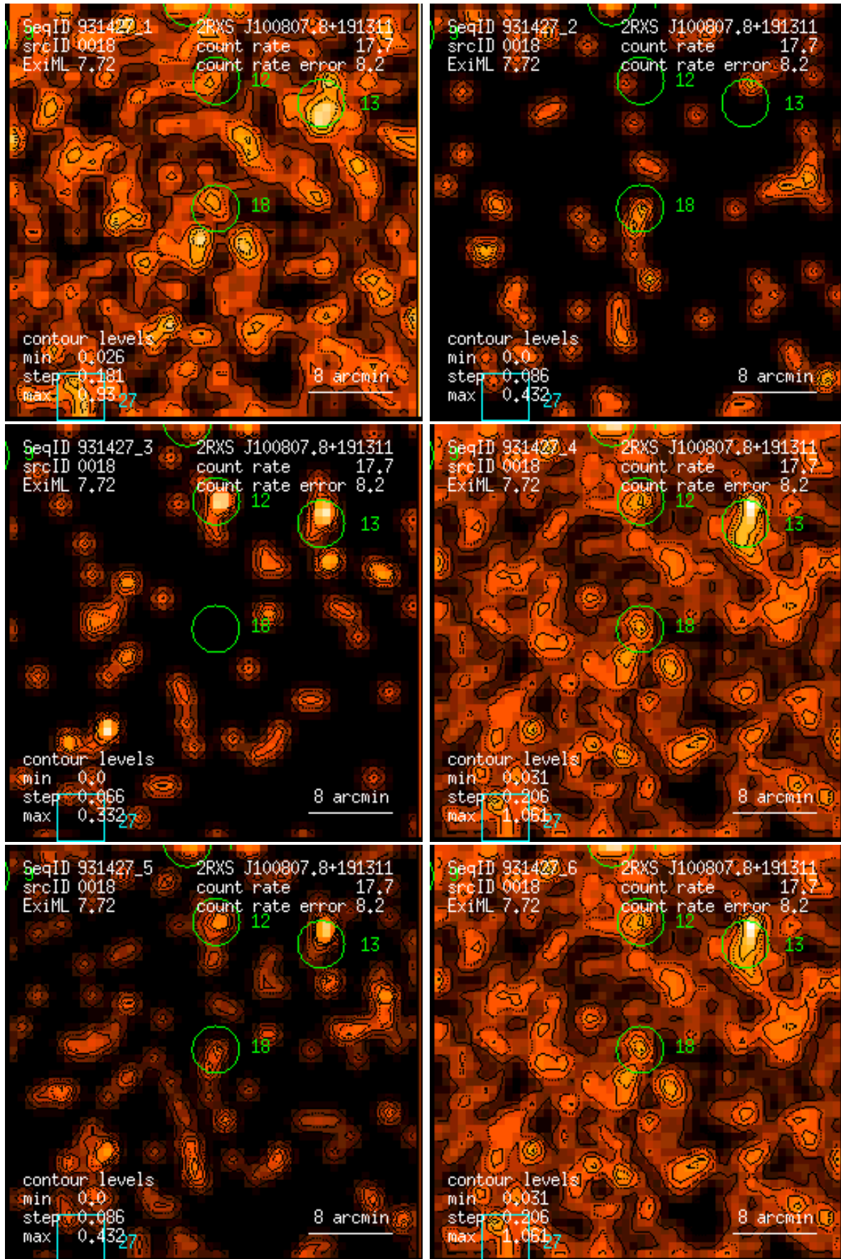
Figure 18: RASS 931427: detection 0018: band rate images, Gaussian filter: (1) PSPC channels 11 – 41, (2) 52 – 90, (3) 91 – 201, (4) 11 – 235, (5) 52 – 201, (6) 11 – 201. Broad band rates in counts/ks. Band rate contour levels in counts/ks/arcmin 2 .
