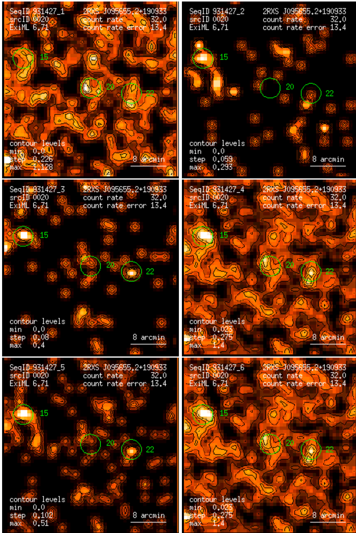
Figure 20: RASS 931427: detection 0020: band rate images, Gaussian filter: (1) PSPC channels 11 – 41, (2) 52 – 90, (3) 91 – 201, (4) 11 – 235, (5) 52 – 201, (6) 11 – 201. Broad band rates in counts/ks. Band rate contour levels in counts/ks/arcmin 2 .
