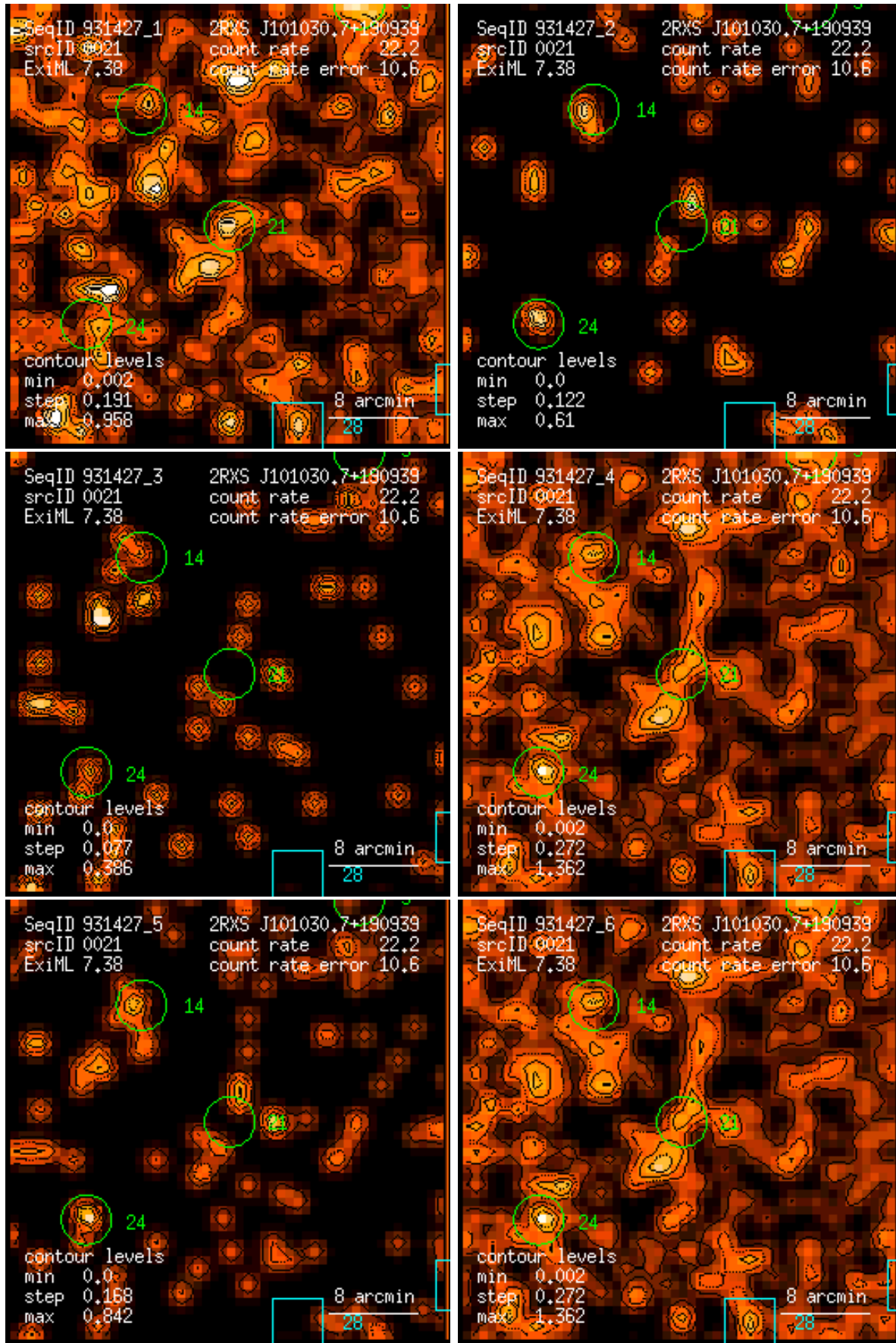
Figure 21: RASS 931427: detection 0021: band rate images, Gaussian filter: (1) PSPC channels 11 – 41, (2) 52 – 90, (3) 91 – 201, (4) 11 – 235, (5) 52 – 201, (6) 11 – 201. Broad band rates in counts/ks. Band rate contour levels in counts/ks/arcmin 2 .
