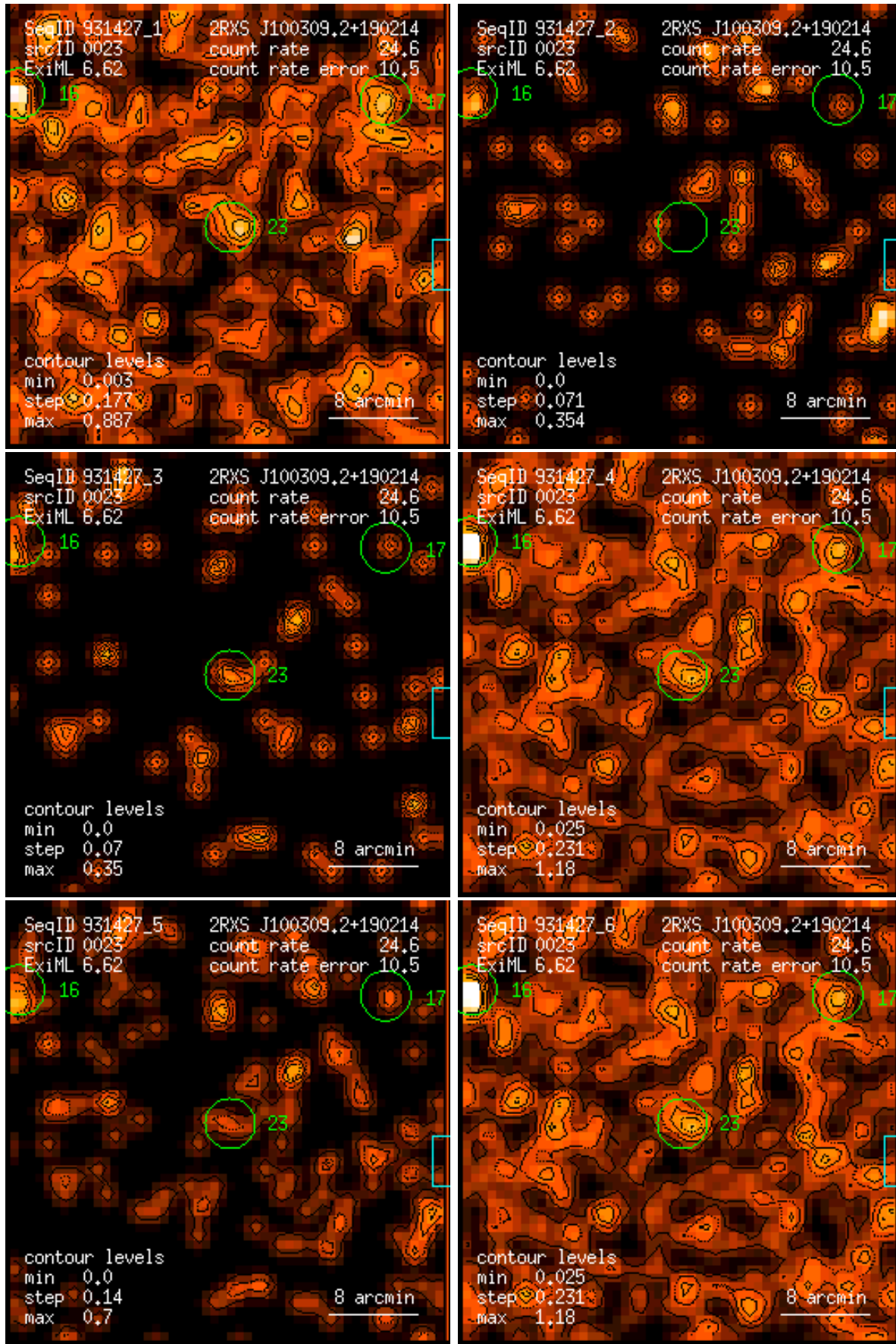
Figure 23: RASS 931427: detection 0023: band rate images, Gaussian filter: (1) PSPC channels 11 – 41, (2) 52 – 90, (3) 91 – 201, (4) 11 – 235, (5) 52 – 201, (6) 11 – 201. Broad band rates in counts/ks. Band rate contour levels in counts/ks/arcmin 2 .
