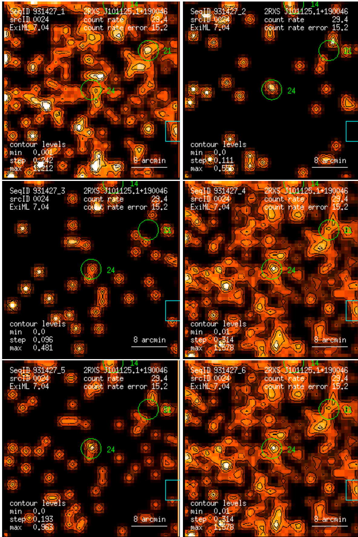
Figure 24: RASS 931427: detection 0024: band rate images, Gaussian filter: (1) PSPC channels 11 – 41, (2) 52 – 90, (3) 91 – 201, (4) 11 – 235, (5) 52 – 201, (6) 11 – 201. Broad band rates in counts/ks. Band rate contour levels in counts/ks/arcmin 2 .
