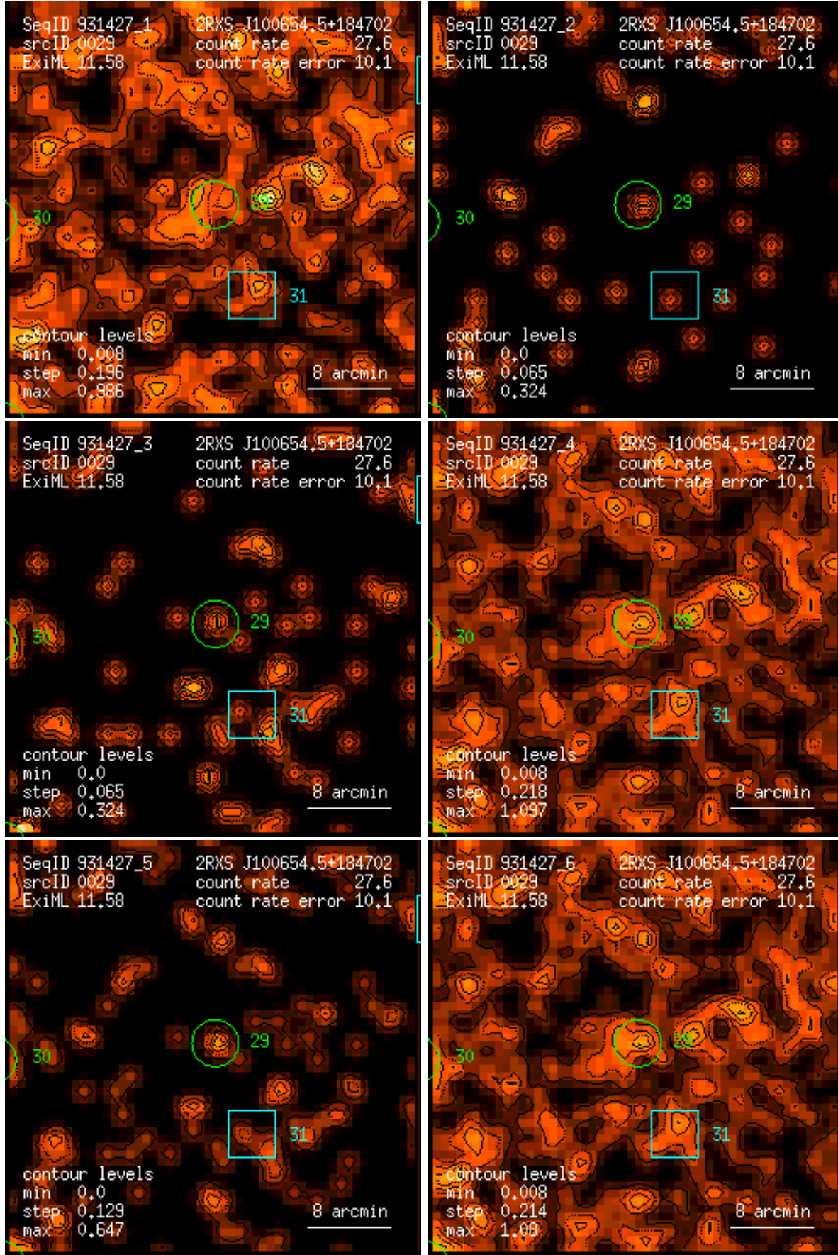
Figure 29: RASS 931427: detection 0029: band rate images, Gaussian filter: (1) PSPC channels 11 – 41, (2) 52 – 90, (3) 91 – 201, (4) 11 – 235, (5) 52 – 201, (6) 11 – 201. Broad band rates in counts/ks. Band rate contour levels in counts/ks/arcmin 2 .
